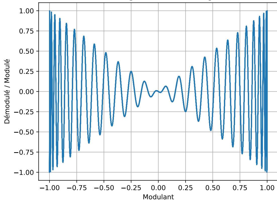
DSB-SC — X-Y : signal modulant vs signal modulé
