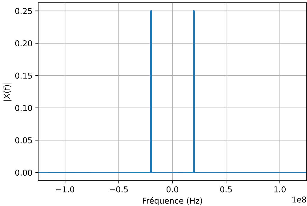
Spectre du signal DSB-SC
