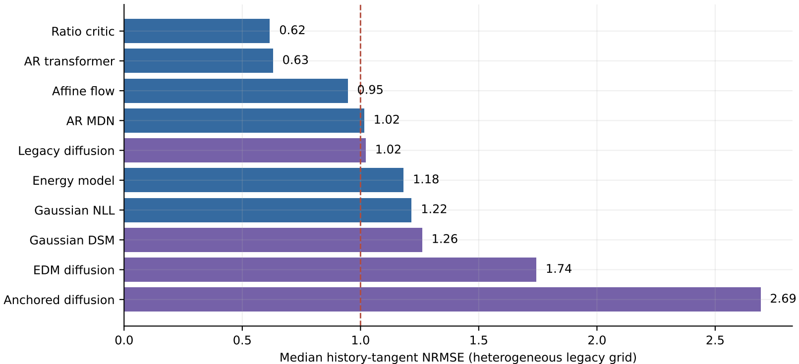
Earlier score/generative benchmark: stable training did not imply a reliable tangent
