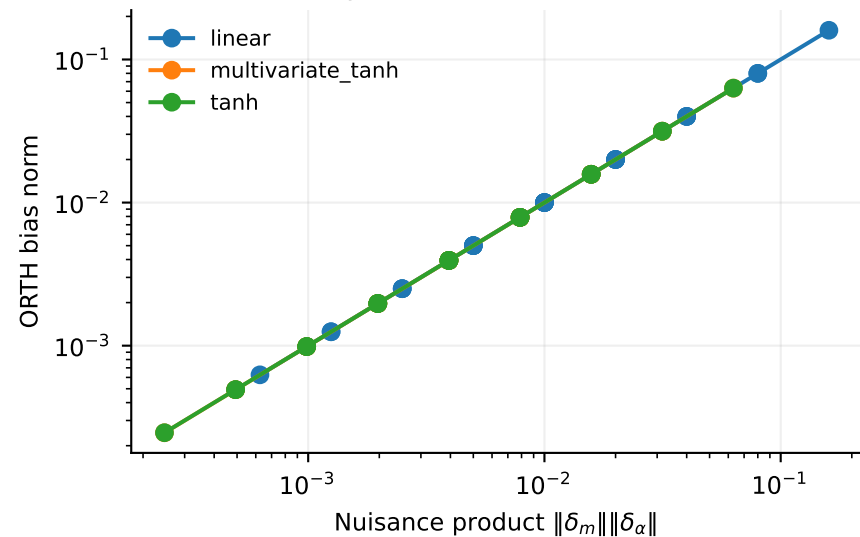
E2: product-order remainder
