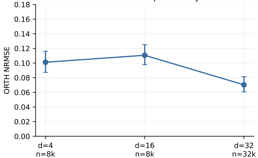
E3: one future per history
