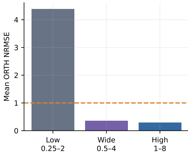
Development frequency audit
