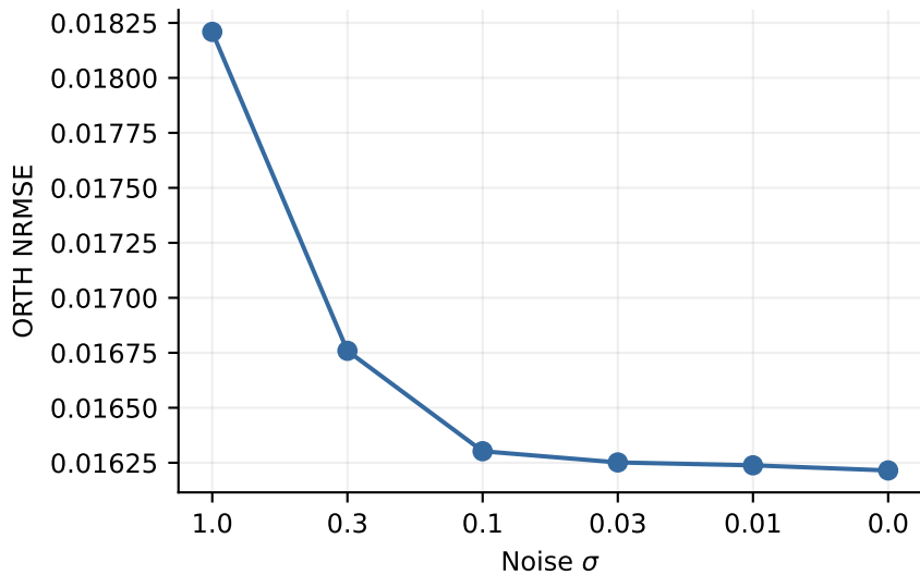
Weak-feature estimator
