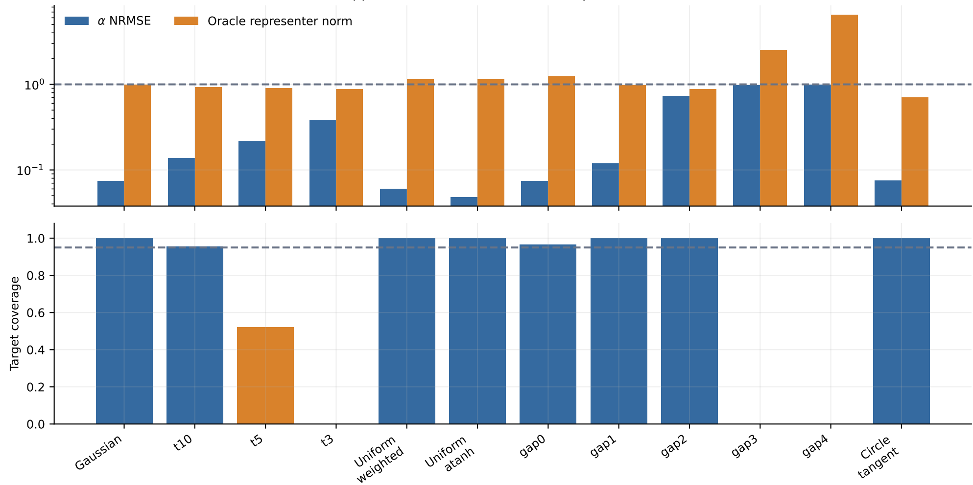
E6: approximation fails as tails/overlap become difficult
