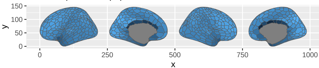
CMrGlu (Neuromaps)
