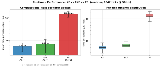
Fig. 3: Measured per-update runtime (mean bar with std whiskers, log scale; right: per-tick distribution) annotated with the per-update asymptotic complexity. d = state dim (3), m = measurement dim (2), M = particles (500).
