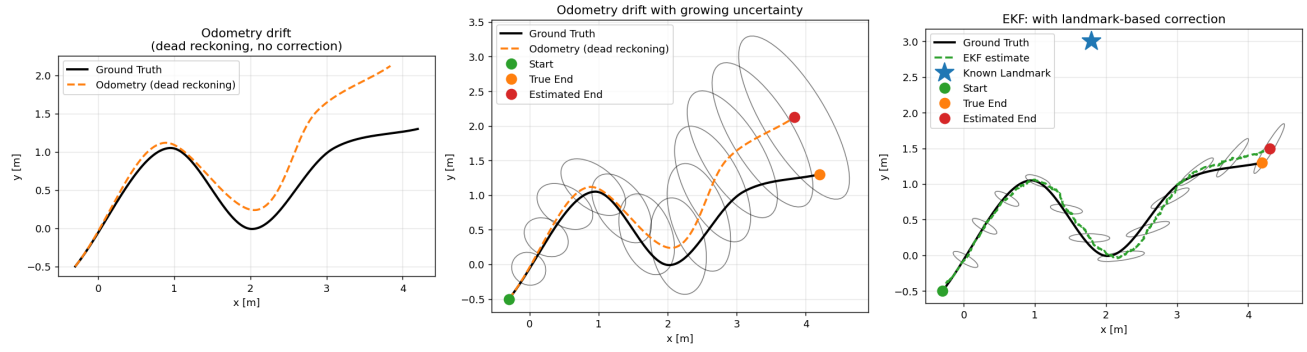
Fig. 3: EKF localization on the S-slalom. Left: odometry drift without corrections. Centre: growing uncertainty (dead-reckoning only). Right: EKF estimate with landmark-based correction; the known landmark (star) keeps the estimate on the true path.
