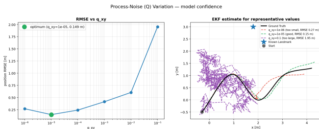
Fig. 8: Process-noise ( Q ) variation. Left: RMSE versus q_{xy} with the optimum marked. Right: EKF estimate for representative values (too small, good, too large).
