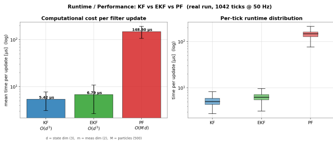
Fig. 3: Measured per-update runtime (mean bar with std whiskers, log scale; right: per-tick distribution) annotated with the per-update asymptotic complexity. d = state dim (3), m = meas dim (2), M = particles (500).
