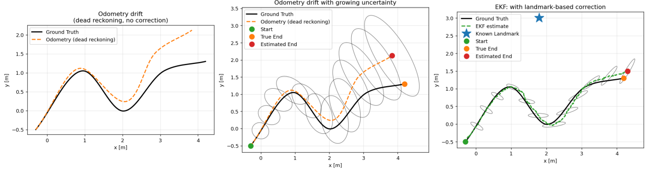
Fig. 4: EKF localization on the S-slalom. Left: odometry drift without corrections. Centre: growing uncertainty (dead-reckoning only). Right: EKF estimate with landmark-based correction; the known landmark (star) keeps the estimate on the true path.
