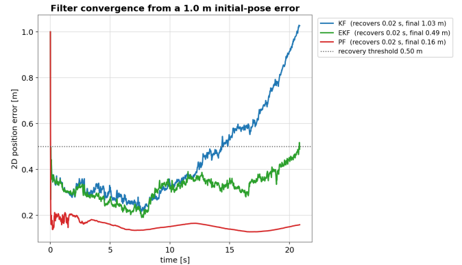
Fig. 10: Convergence from a 1.0 m initial-pose error (12-seed mean position error over time). The PF recovers and stays low; the EKF holds; the KF recovers then destabilises.
