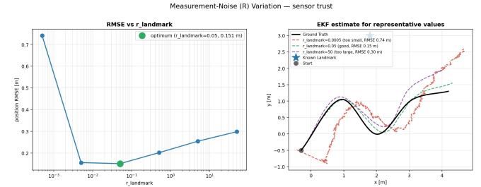
Fig. 9: Measurement-noise ( R ) variation. Left: RMSE versus r with the optimum marked. Right: EKF estimate for representative values.
