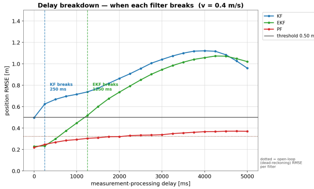
Fig. 7: Delay breakdown: position RMSE versus measurement delay (12-seed mean) with each filter's breaking point (first delay with RMSE > 0.5 m). Dotted lines mark the open-loop (dead-reckoning) RMSE per filter.
