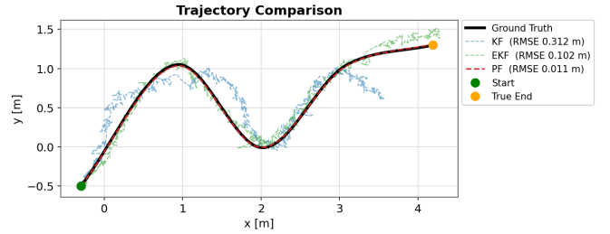
Fig. 1: Trajectory comparison on the S-slalom: Ground Truth (black), KF (blue dashed), EKF (green dashed), and PF (red dashed, tracking tightly under the ground-truth line).
