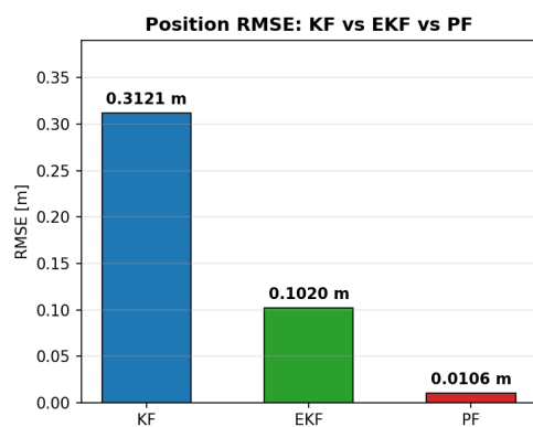
Fig. 11: Baseline position RMSE for KF, EKF and PF on the S-slalom.
