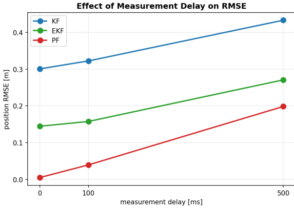
Fig. 5: Position RMSE versus measurement-processing delay for KF, EKF and PF. All filters degrade monotonically with delay.
