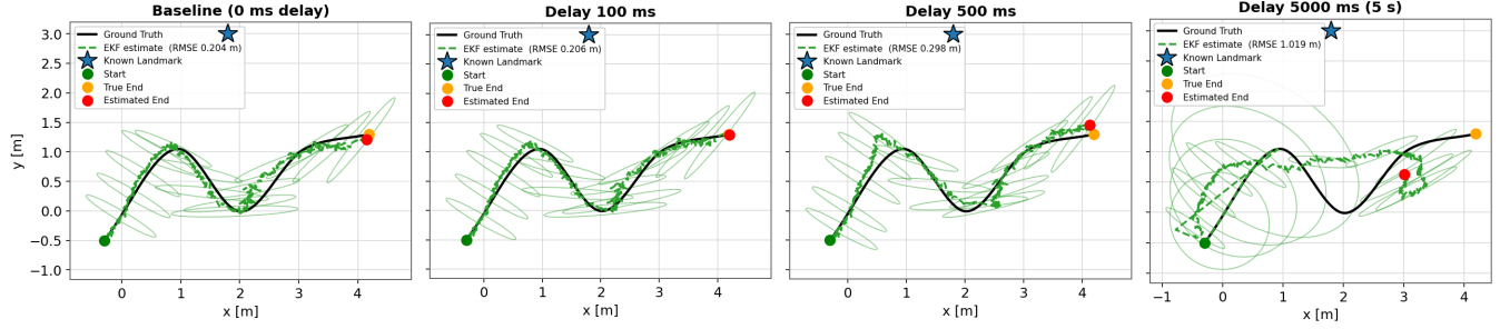
Fig. 6: EKF estimate on the S-slalom under increasing measurement-processing delay (0, 100, 500 and 5000 ms): Ground Truth (black), EKF estimate (green dashed) with 2\sigma covariance ellipses, and the known landmark (blue star). RMSE (averaged over 30 noise realisations) grows with delay; at 5 s the stale correction no longer matches the current pose and the estimate diverges from the track (RMSE \approx 1.0 m).
