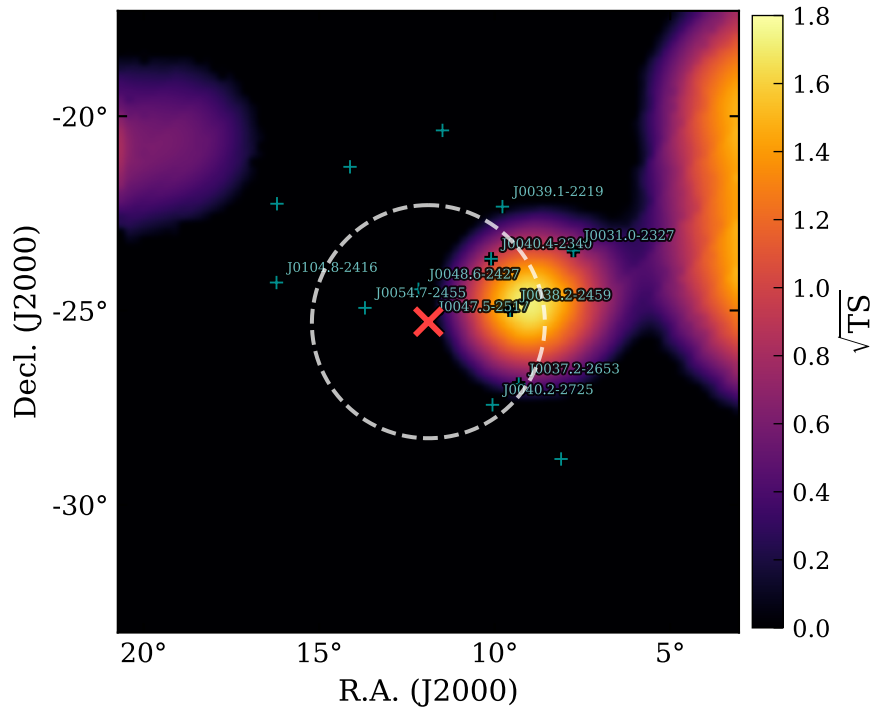
\sqrt{\text{TS}} (GRB081213A in model)
