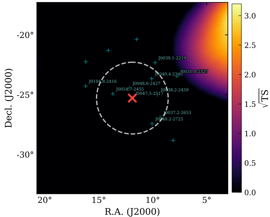
\sqrt{\text{TS}} (GRB180128A in model)
