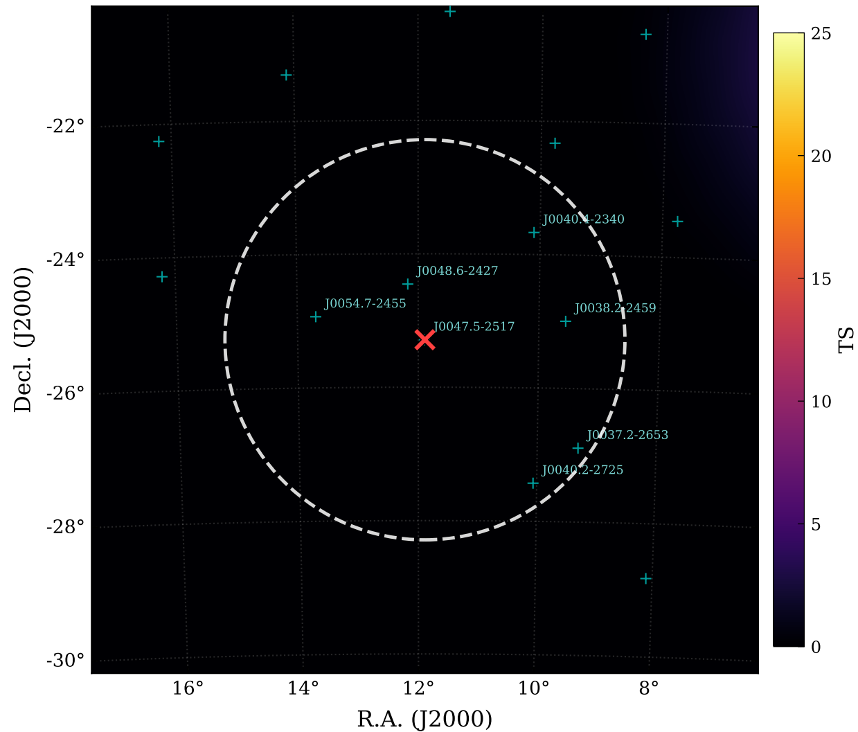
without GRB180128A in model
