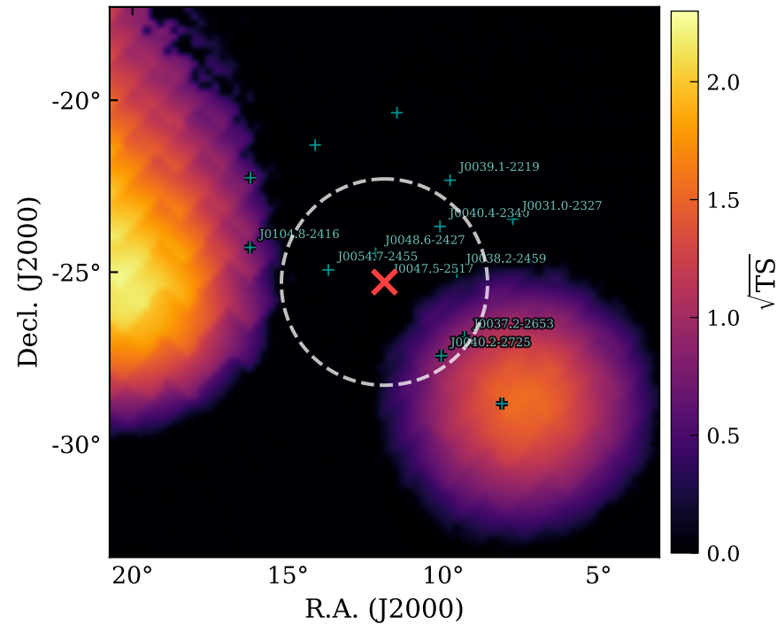
\sqrt{\text{TS}} (no GRB231024A)
