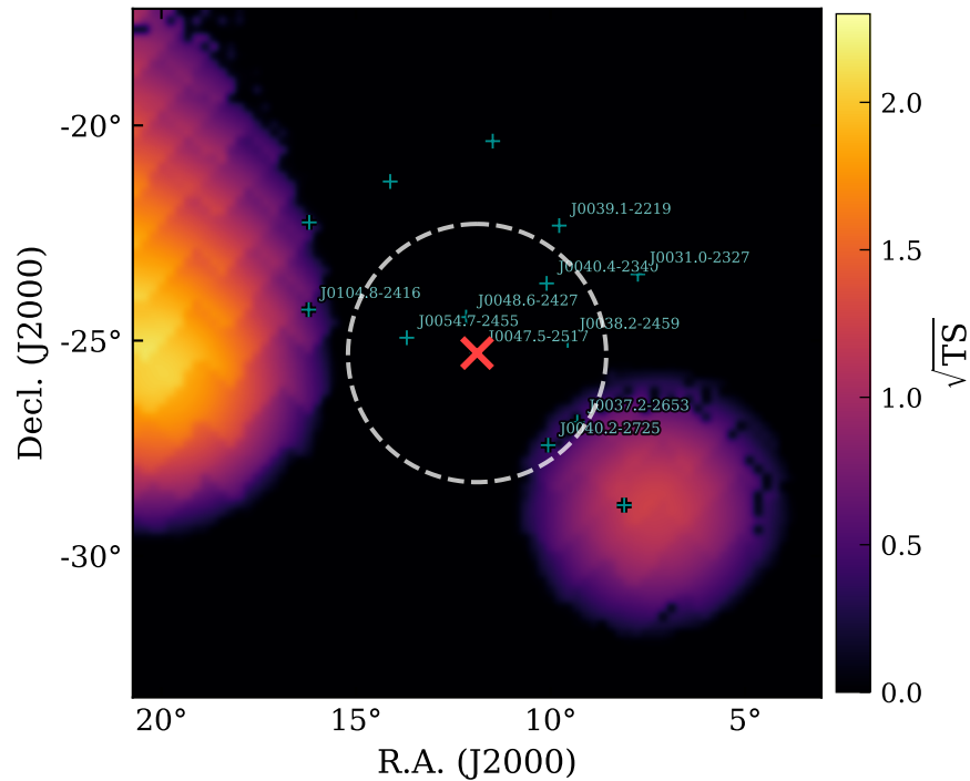
\sqrt{\text{TS}} (GRB231024A in model)
