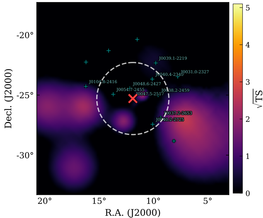
\sqrt{\text{TS}} (GRB200415A in model)
