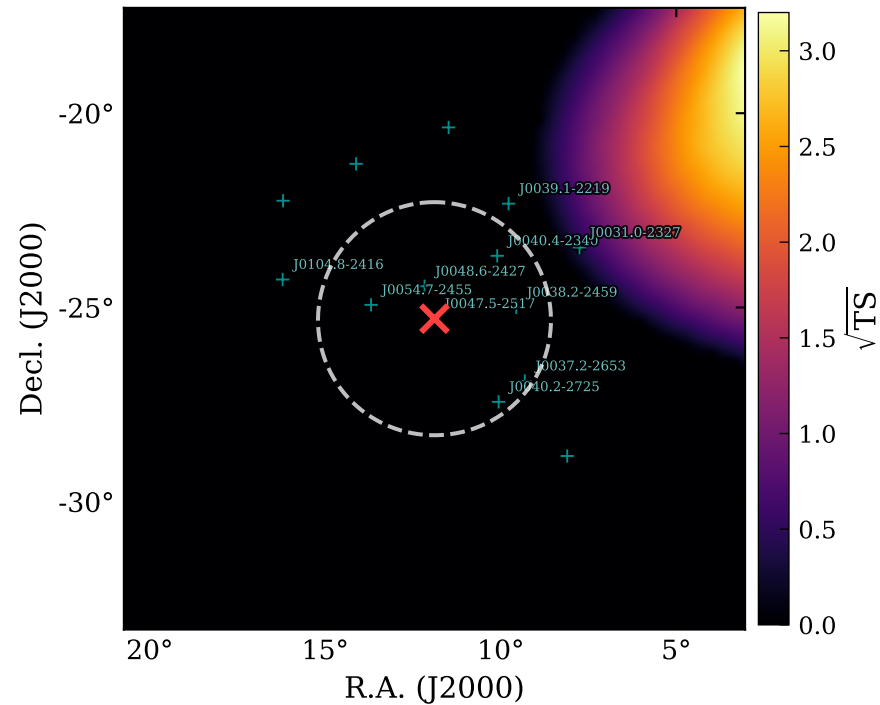
\sqrt{\text{TS}} (no GRB180128A)
