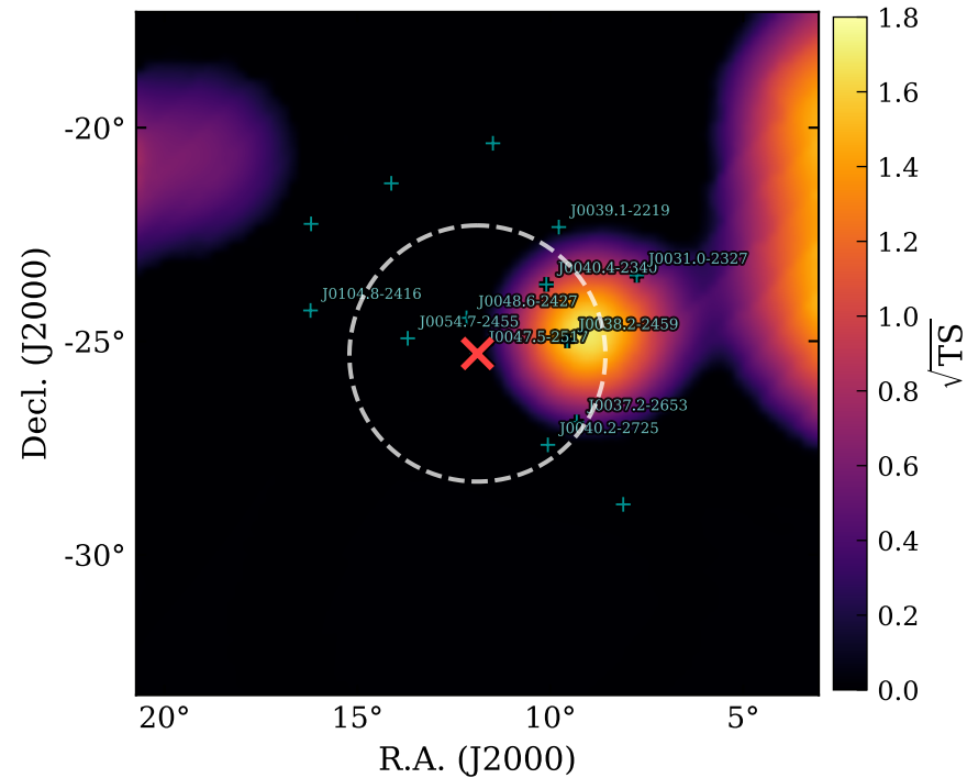
\sqrt{\text{TS}} (no GRB081213A)
