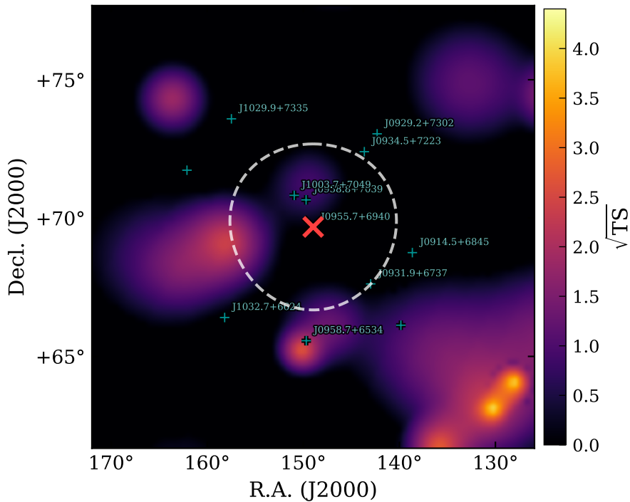
\sqrt{\text{TS}} (GRB231115A in model)
