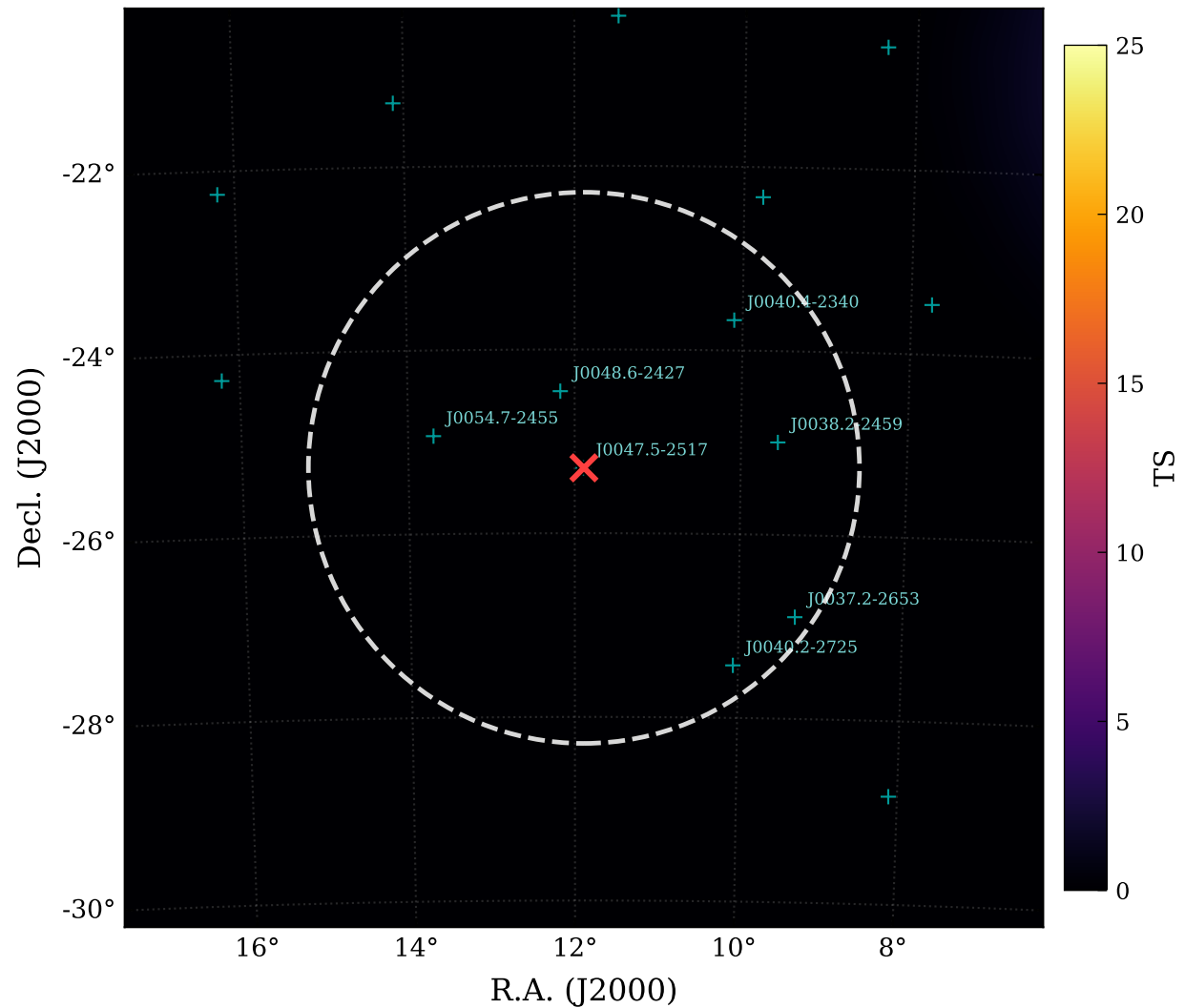
GRB180128A in model
