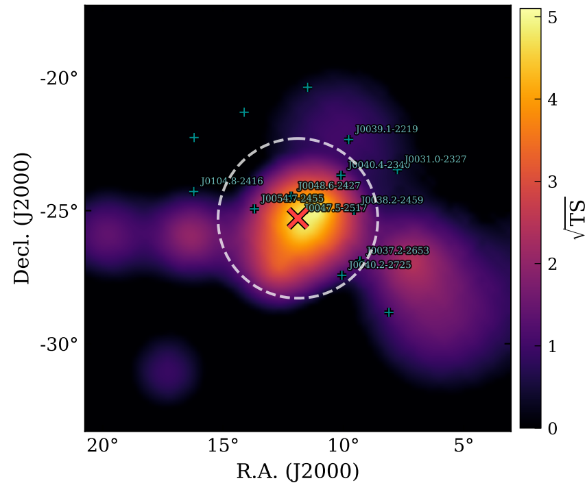
\sqrt{\text{TS}} (no GRB200415A)
