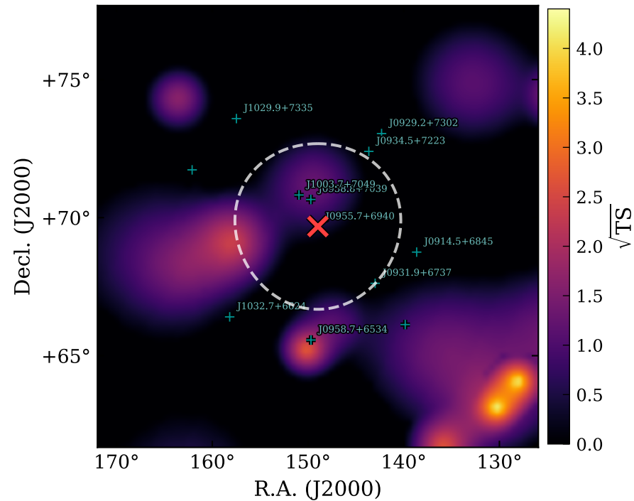
\sqrt{\text{TS}} (no GRB231115A)
