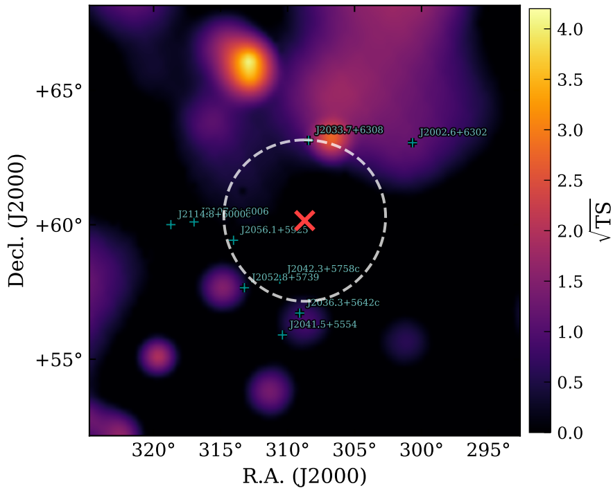
\sqrt{\text{TS}} (GRB200423A in model)
