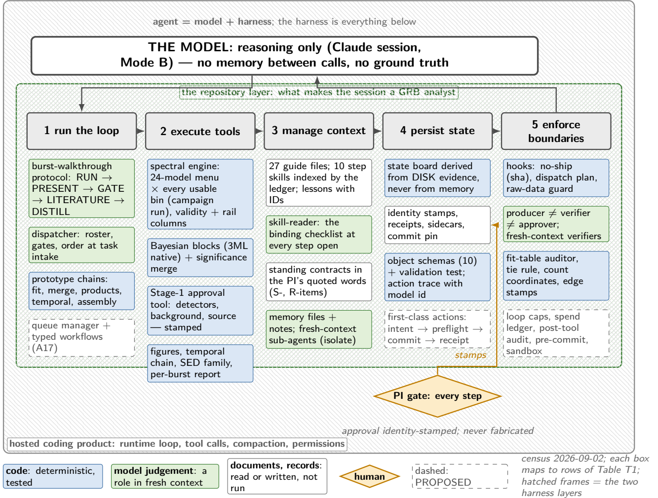
Figure 1. The harness anatomy. The five runtime jobs of an agent harness, with the components this campaign has under each. Colour says what executes: blue boxes are deterministic code, green boxes are roles the language model plays in a fresh context, white boxes are documents and records that are read or written but not run, and the amber diamond is the human. Solid boxes satisfy the roster’s file-or-recorded-product convention in the census working tree; dashed boxes are proposed in the requirements register and not built. The two hatched frames are the two harness layers: the hosted coding product outside, the repository inside. The protocol requires every gate to carry an approver identity; stamp coverage is not yet complete across the sample, and Stage-1 approvals may be human or AI, stamped either way. Each box maps to rows of Table 2.
