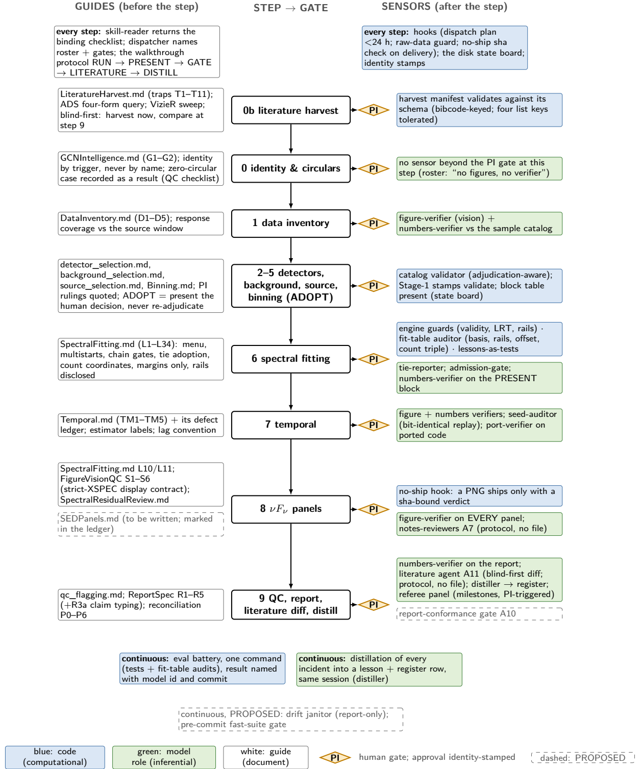
Figure 2. The per-burst lifecycle with its guides and sensors. Centre: the eleven ledger steps, top to bottom, each followed by the human gate. Left: the guides that steer each step before it runs, chiefly the step’s skill document with its numbered lessons and the standing contracts in the human’s words. Right: the sensors that check each step after it runs, blue where the check is code (tests, hooks, the fit-table auditor, schema validation) and green where it is a fresh-context role (figure, numbers, seed, port verifiers; the tie reporter; the admission gate); guides are white, and the amber diamond is the human gate. Below the ledger, the checks that run continuously. Dashed items are proposed.
