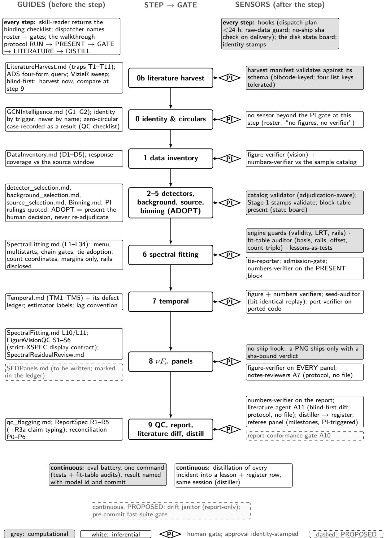
Figure 2. The per-burst lifecycle with its guides and sensors. Centre: the eleven ledger steps, top to bottom, each followed by the human gate. Left: the guides that steer each step before it runs, chiefly the step’s skill document with its numbered lessons and the standing contracts in the human’s words. Right: the sensors that check each step after it runs, grey where the check is code (tests, hooks, the fit-table auditor, schema validation) and white where it is a fresh-context role (figure, numbers, seed, port verifiers; the tie reporter; the admission gate). Below the ledger, the checks that run continuously. Dashed items are
