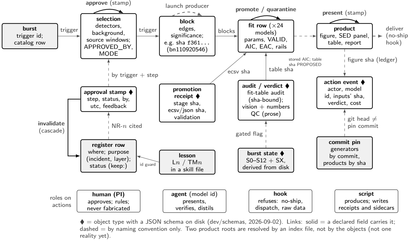
Figure 5. The object-and-action model. Top row: the burst’s chain of products, from trigger to report. Middle row: the records about those products. Bottom row: the law that governs them. A diamond marks an object type with a JSON schema on disk. Links are solid where a declared field carries them (a trigger key, a content hash, a commit) and dashed where they hold by naming convention. Actions are labelled arrows, solid where they are first-class on disk today and dashed where proposed. The band beneath names the four roles that act. Every box maps to rows of Table 2.
