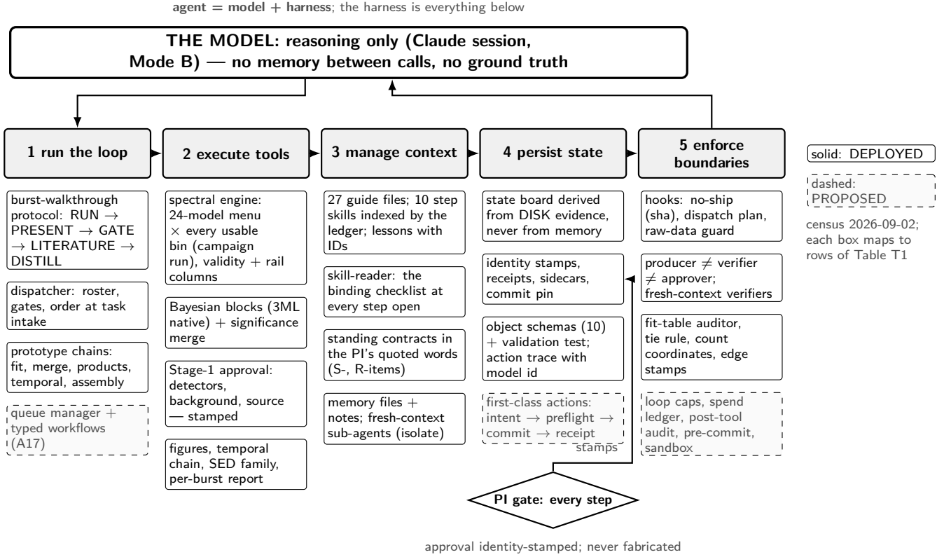
Figure 1. The harness anatomy. The five runtime jobs of an agent harness, with the components this campaign has under each. Solid boxes satisfy the roster’s file-or-recorded-product convention in the census working tree; dashed boxes are proposed in the requirements register and not built. The protocol requires every gate to carry an approver identity; stamp coverage is not yet complete across the sample, and Stage-1 approvals may be human or AI, stamped either way. Each box maps to rows of Table 2.
