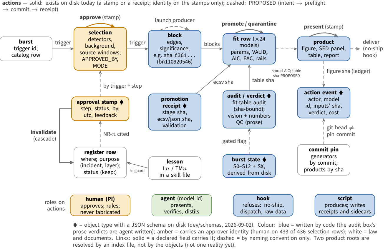
Figure 6. The object-and-action model. Top row: the burst’s chain of products, from trigger to report. Middle row: the records about those products. Bottom row: the law that governs them. Colour says who writes the object: blue by code (the audit box also holds the agent-written vision and numbers verdicts), amber carrying an approver identity (human on 433 of the 436 selection rows), white the law and documents; the roles band uses the same colours, green for the agent. A diamond marks an object type with a JSON schema on disk. Links are solid where a declared field carries them (a trigger key, a content hash, a commit) and dashed where they hold by naming convention. Actions are labelled arrows, solid where they are first-class on disk today and dashed where they are proposed. The band beneath names the four roles that act. Every box maps to rows of Table 4.
