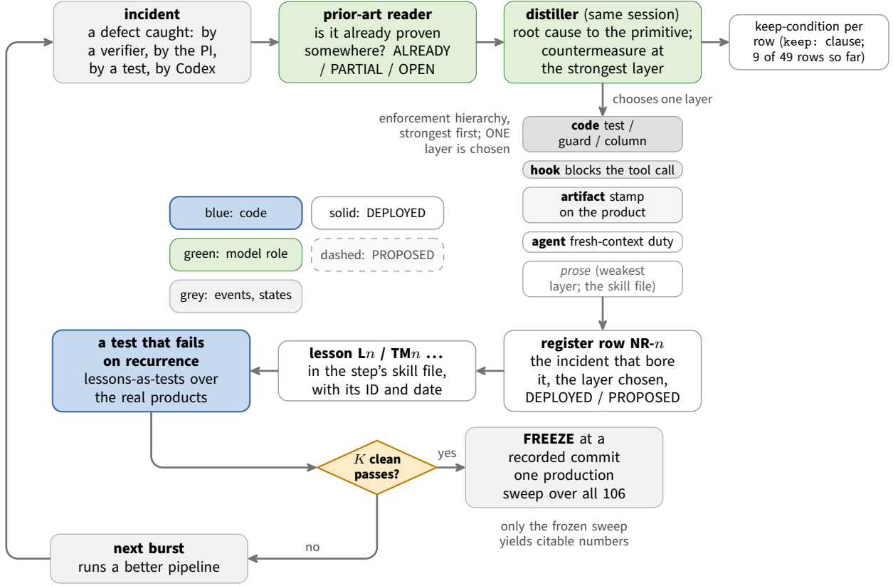
Figure 4. The steering loop. An incident, caught by a verifier, a test, the external auditor, or the human, passes a prior-art reader and a distiller (green: model roles) that place the countermeasure at the strongest layer of the enforcement ladder (grey rungs, graded by strength), then record it as a register row and a numbered lesson (white: documents) with a test that fails on recurrence (blue: code). The amber diamond is the human’s decision to declare convergence after K clean passes; the freeze and the single production sweep follow. Neither has yet occurred: K is not set and no clean pass has been recorded.
