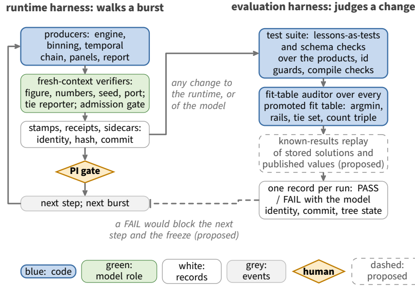
Figure 7. Two harnesses. Left, the runtime harness that walks a burst: producers, fresh-context verifiers, stamps, and the human gate. Right, the evaluation harness that judges a change to the runtime: the test suite, the fit-table auditor over every promoted fit table, and the proposed known-results replay, run as one command whose record carries the model identity, the commit, and the state of the working tree. In the record of 2026 September 3 the suite was 137 tests (136 passed, one expected failure) and the auditor read the fit tables of the twenty-five bursts promoted so far, three of which it flagged. Every change to the runtime harness, and every change of model, is a reason to run the right-hand side, but that trigger is a discipline rather than a hook: the pre-commit gate that would enforce it is proposed. The dashed return, a failed battery blocking the next step and the freeze, is proposed: today the battery records its verdict and nothing yet consumes it.
