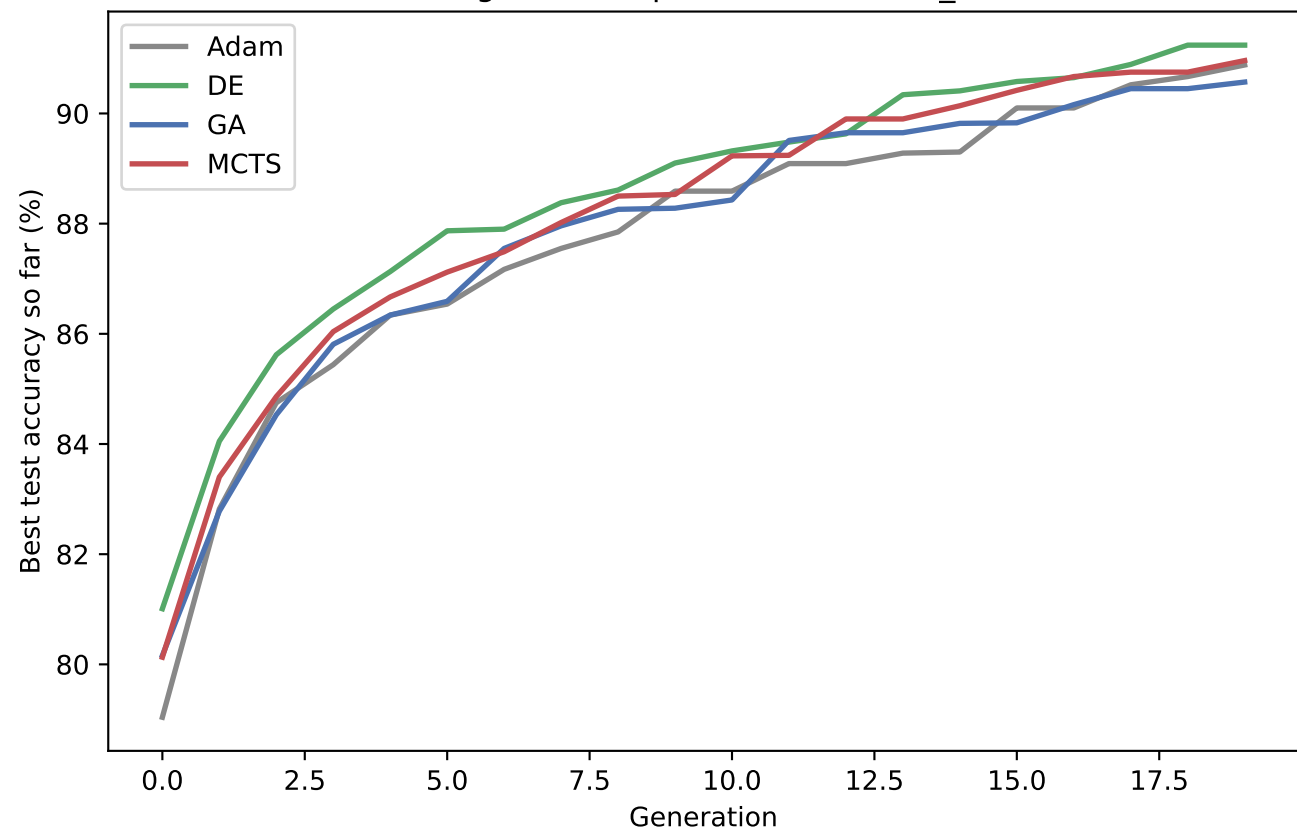
Convergence comparison — fashion_mnist
