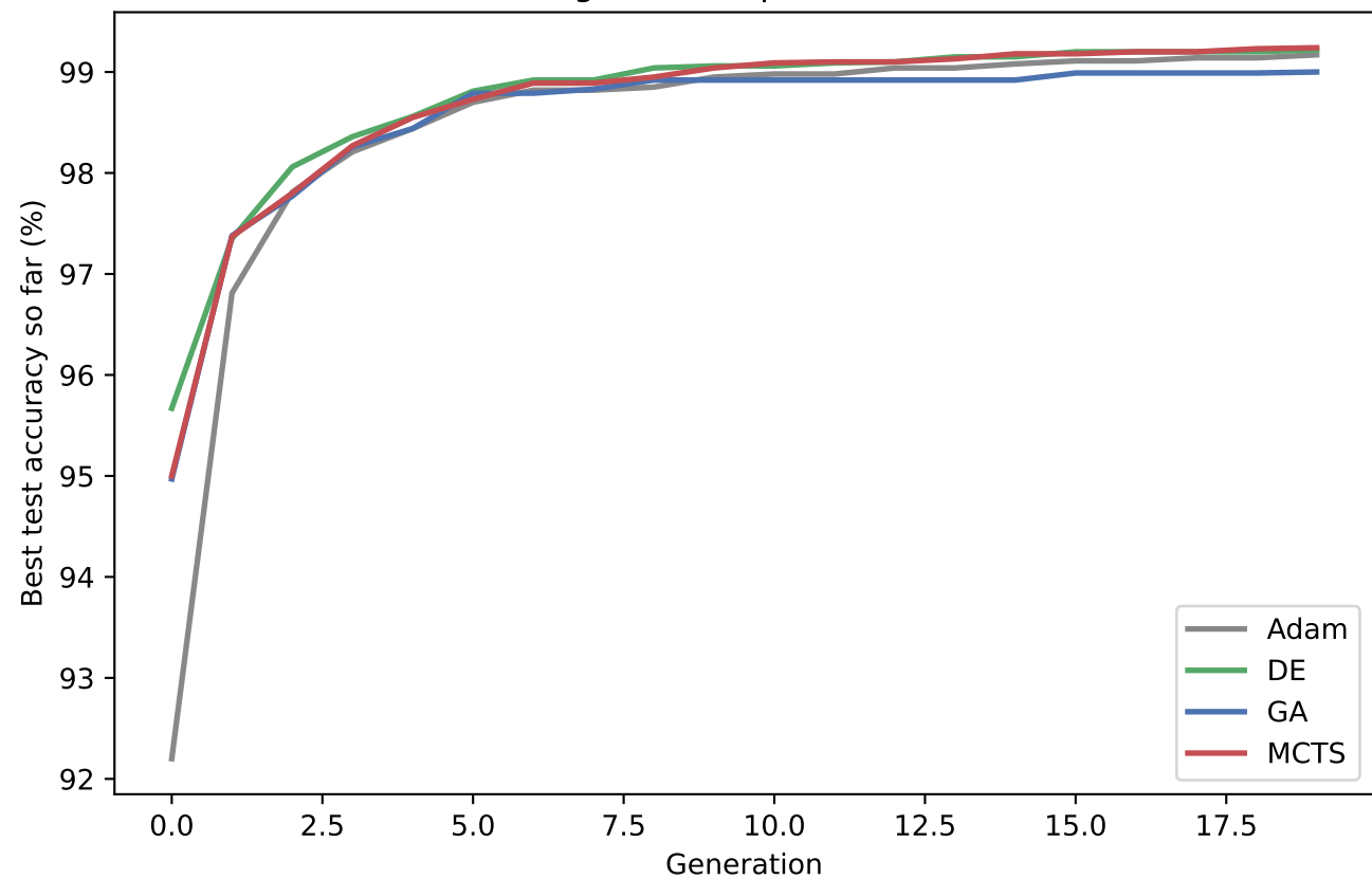
Convergence comparison — mnist
