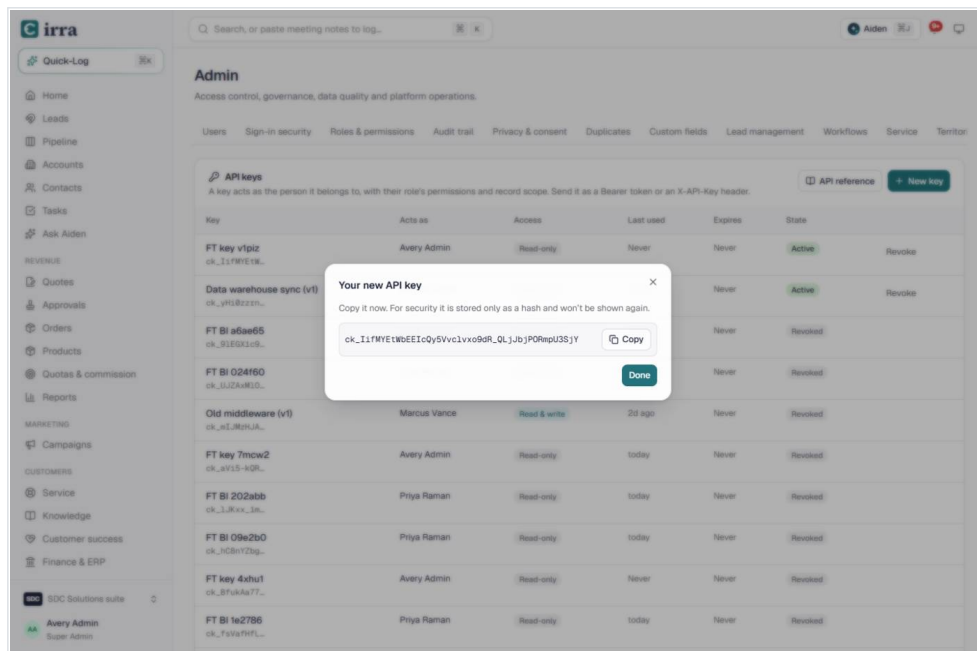
Read-only API key issued once; verified GET 200 / POST 403
