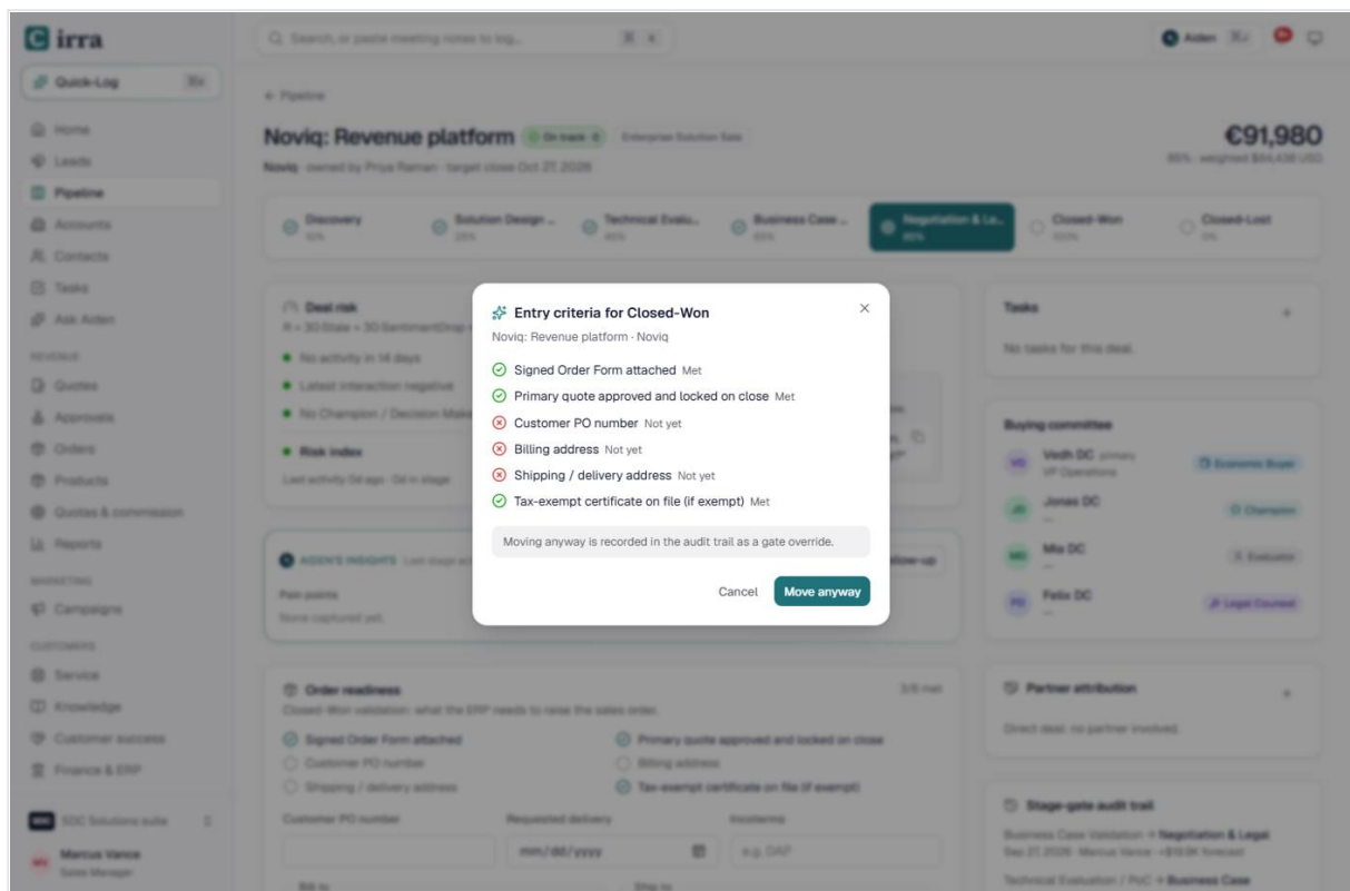
E20 (TC-34) - Closed-Won blocked by the order checks
