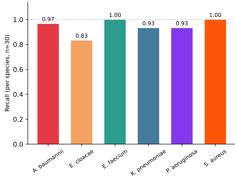
(B) C3 holdout: per-species recall (30 novel-ST-prioritised genomes per species)
