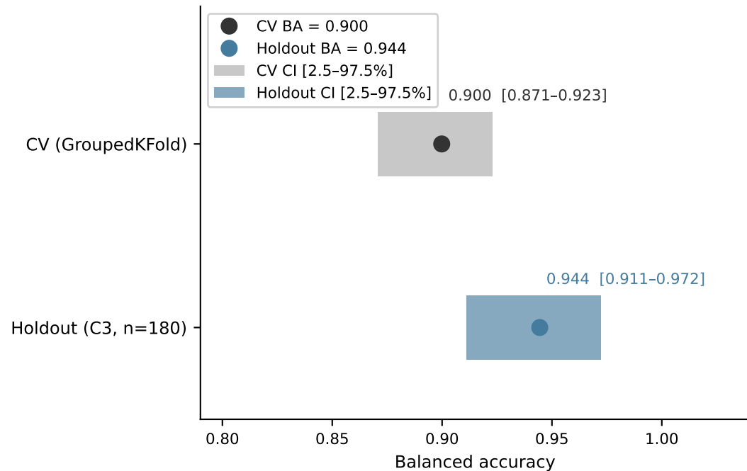
Holdout BA vs CV estimate Consistent: holdout 0.944 [0.911–0.972], CV 0.900 [0.871–0.923]
