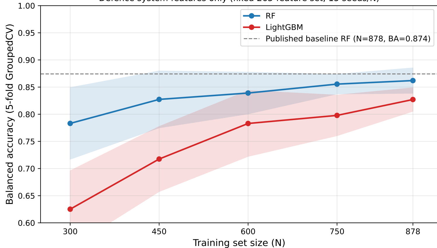
Q1 Learning Curve — ESKAPE species classification Defence system features only (fixed 265-feature set, 15 seeds/N)
