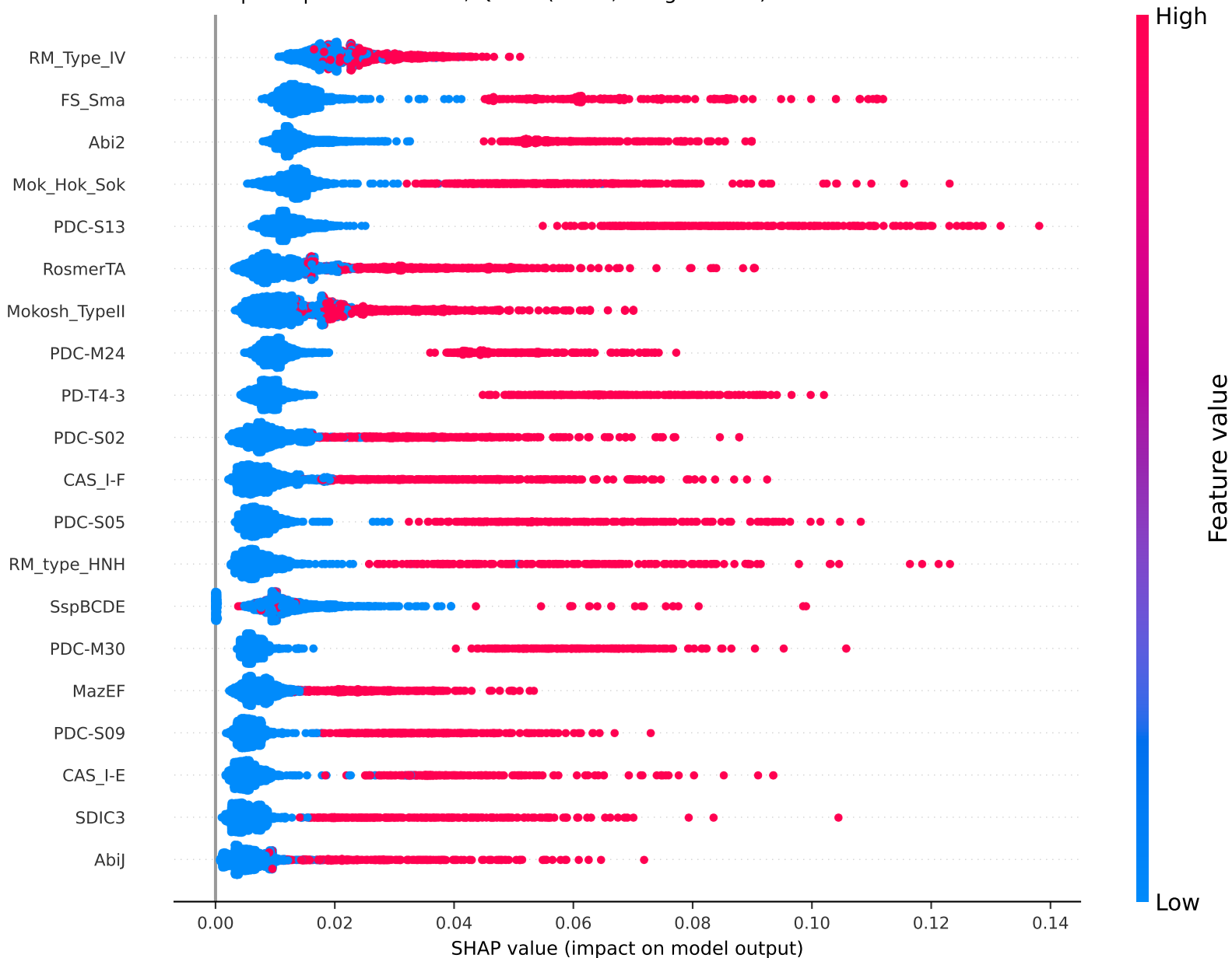
(A) Global SHAP beeswarm — top 20 features mean |SHAP| over 6 classes, Q1 RF (n = 3,335 genomes)
