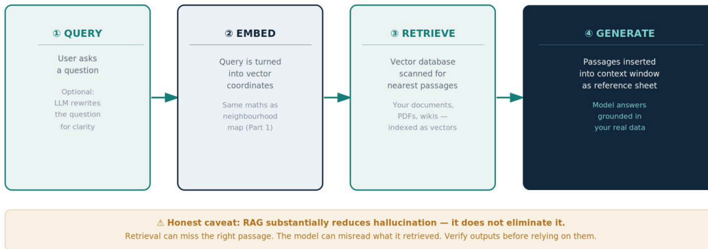
Figure 1: The canonical pipeline has four steps
