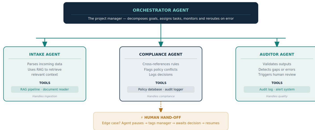
Figure 2: 1. Multi-agent orchestration (the digital manager)
