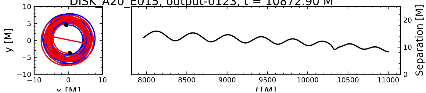
DISK A20 E015, output-0123, t = 10872.90 M
