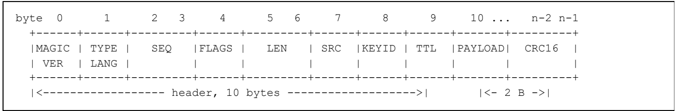
Figure 2.2: Frame format.
