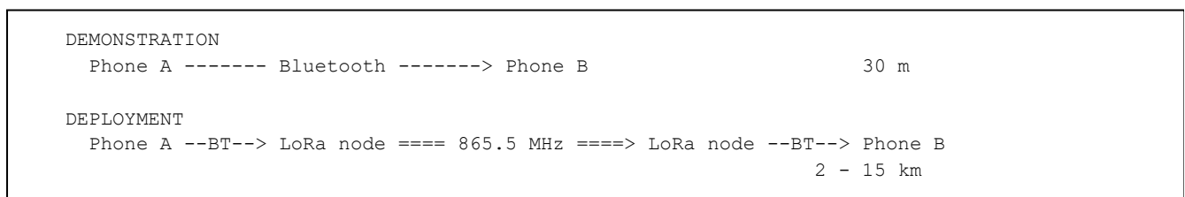
Figure 1.3: The handset software is identical in both topologies. Only what sits at the far end of the Bluetooth connection differs.
