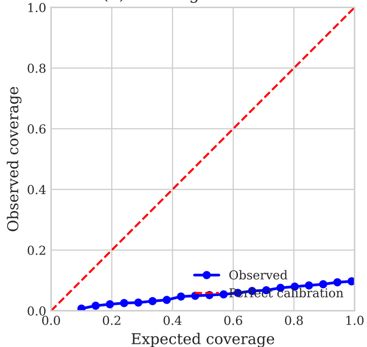
(b) Coverage calibration
