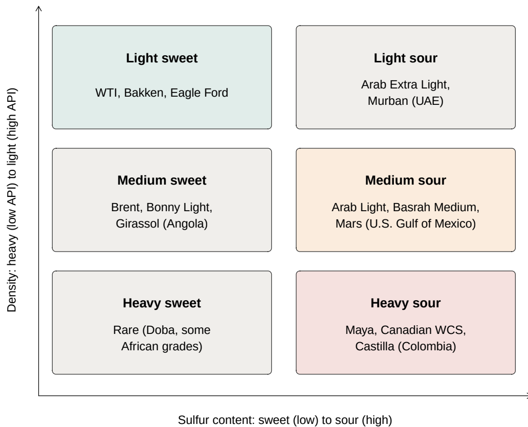
Figure 1: Crude oil categories by density and sulfur content
