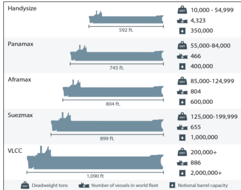
Figure 5: Oil tanker size ranges: world fleet as of 2023
