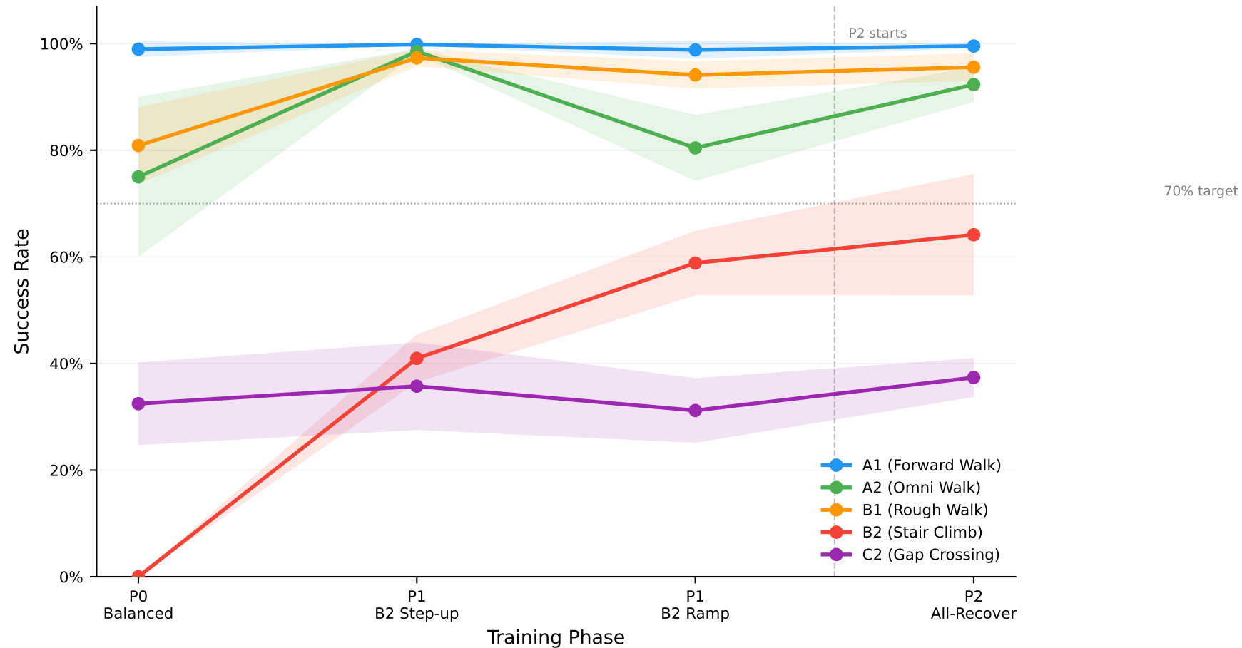
MTL Policy: Per-Task Success Rate Across Training Phases (mean \pm std, n=3 seeds each)
