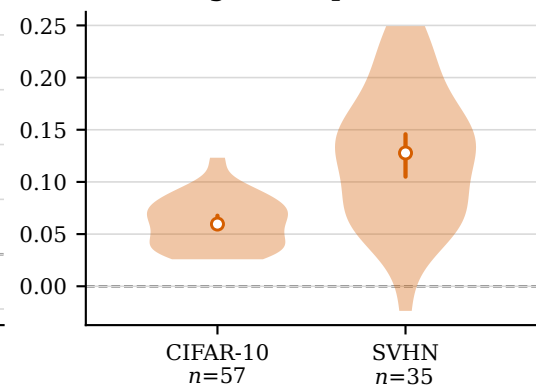
delegators + predictors
