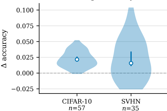
delegators only
