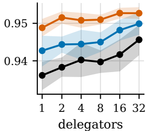
Bike Sharing
