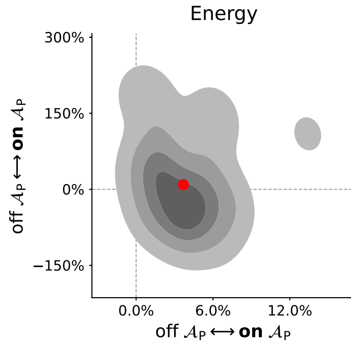
Individual Predictor Performance
