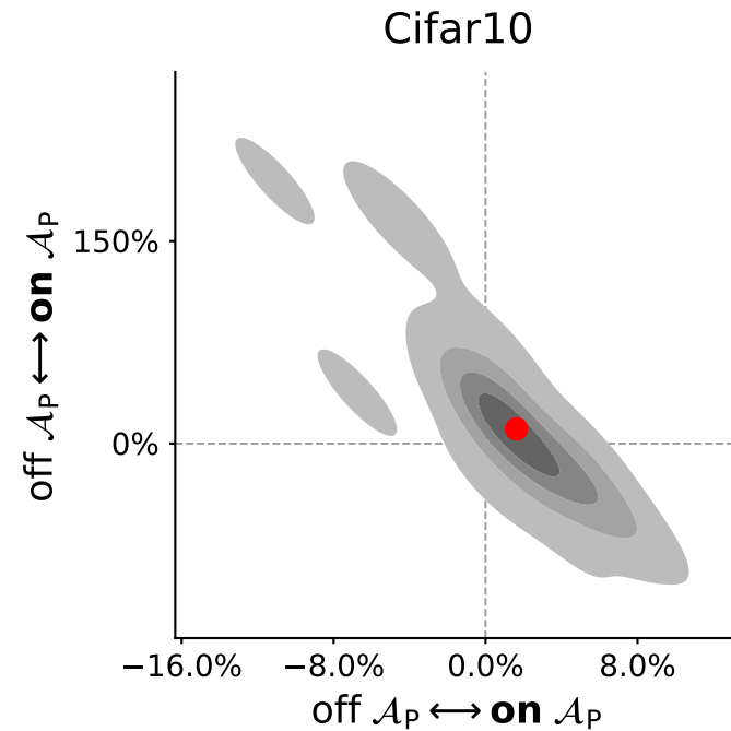
Individual Predictor Performance
