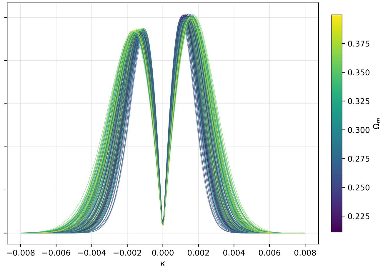
Sim L_1 mean (per cosmology, over 7 perms), \theta=100.0'
