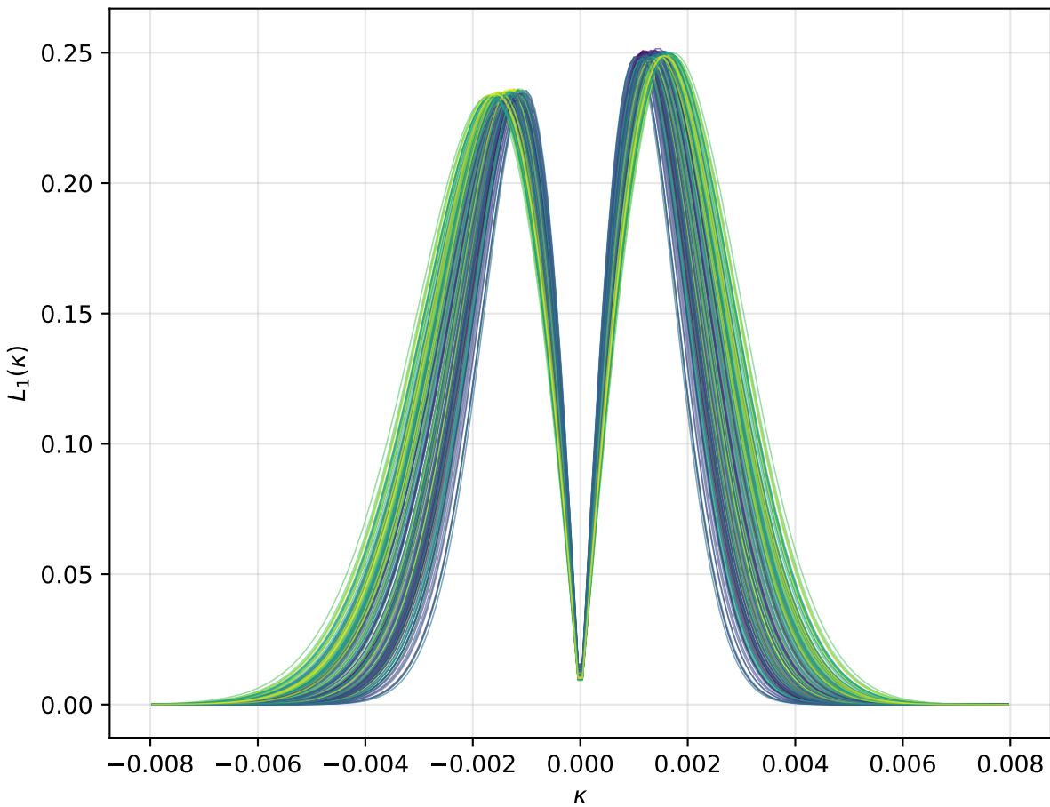
Theory L_1 (per cosmology), \theta=100.0'
