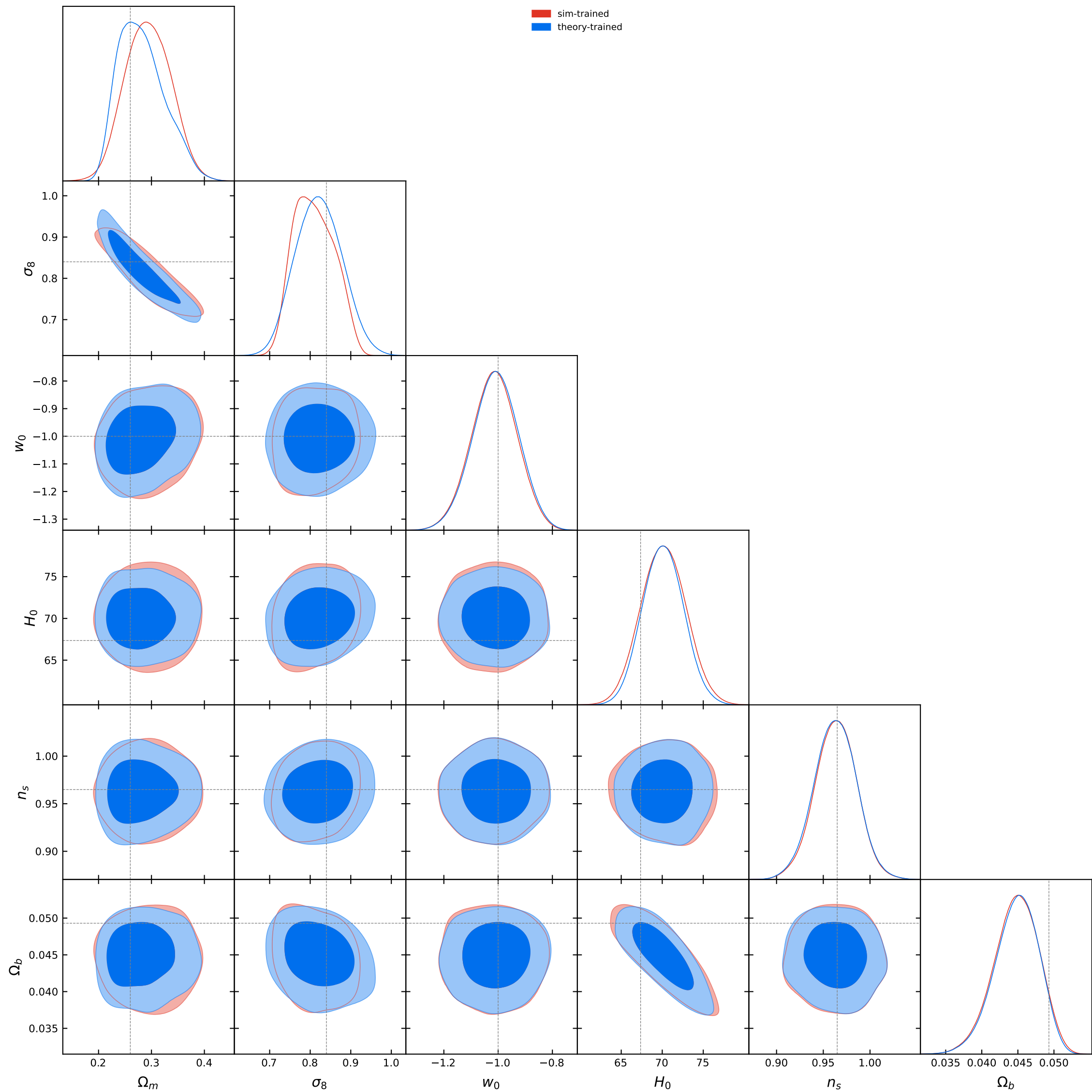
L1 NPE contours: sim vs theory, theta100, cut=aminm0p005_amaxp0p005
