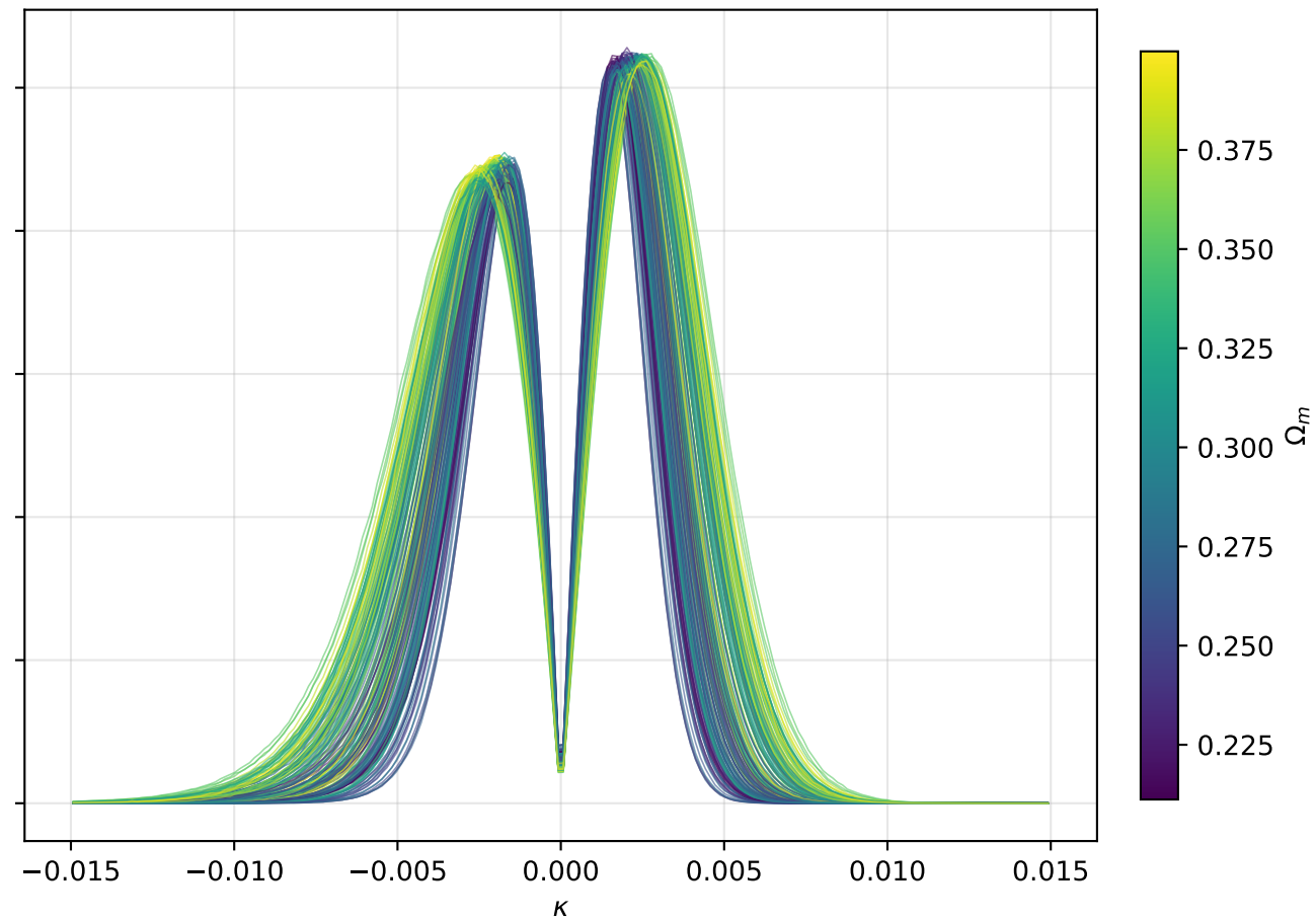
Sim L_1 mean (per cosmology, over 7 perms), \theta=30.0'
