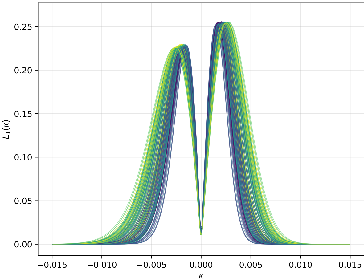
Theory L_1 (per cosmology), \theta=30.0'
