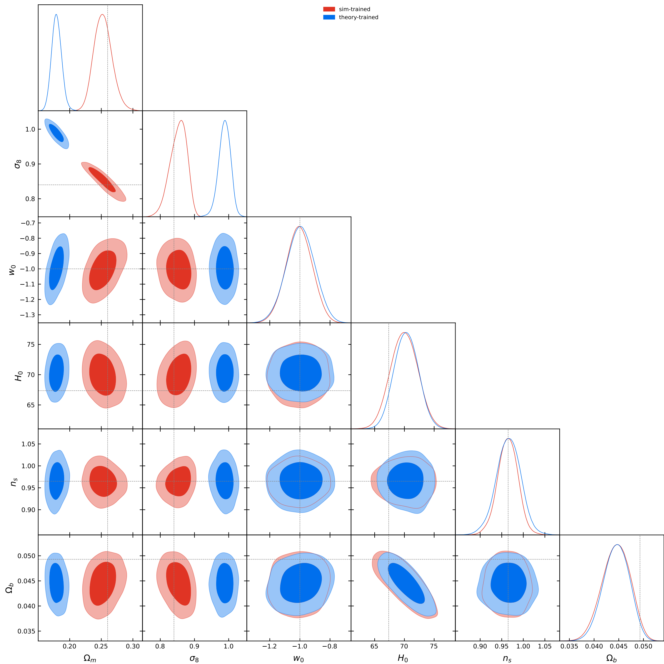
L1 NPE contours: sim vs theory, theta30, cut=aminm0p005_amaxp0p005_dcrm
