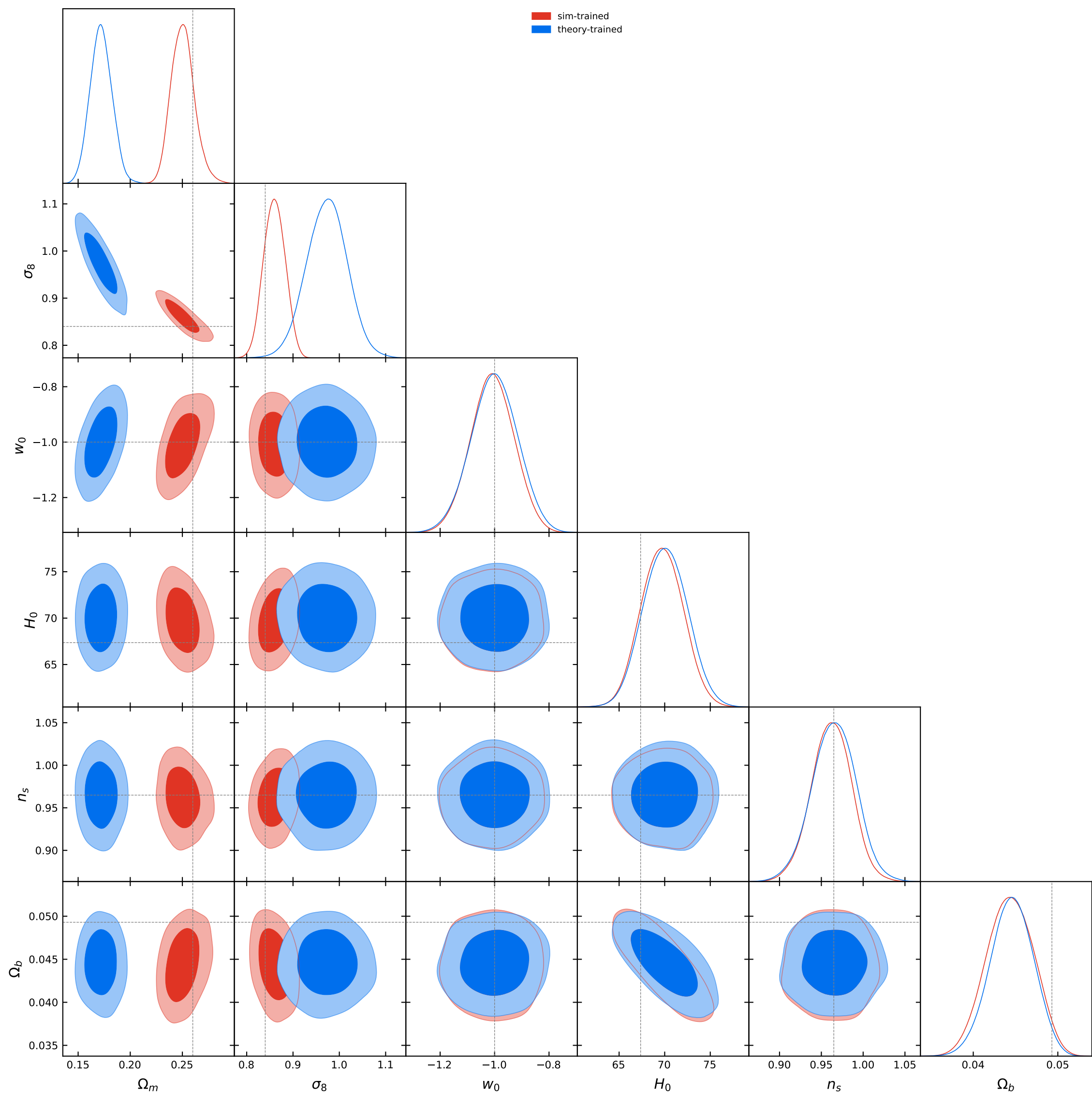
L1 NPE contours: sim vs theory, theta30, cut=aminm0p012_amaxp0p012
