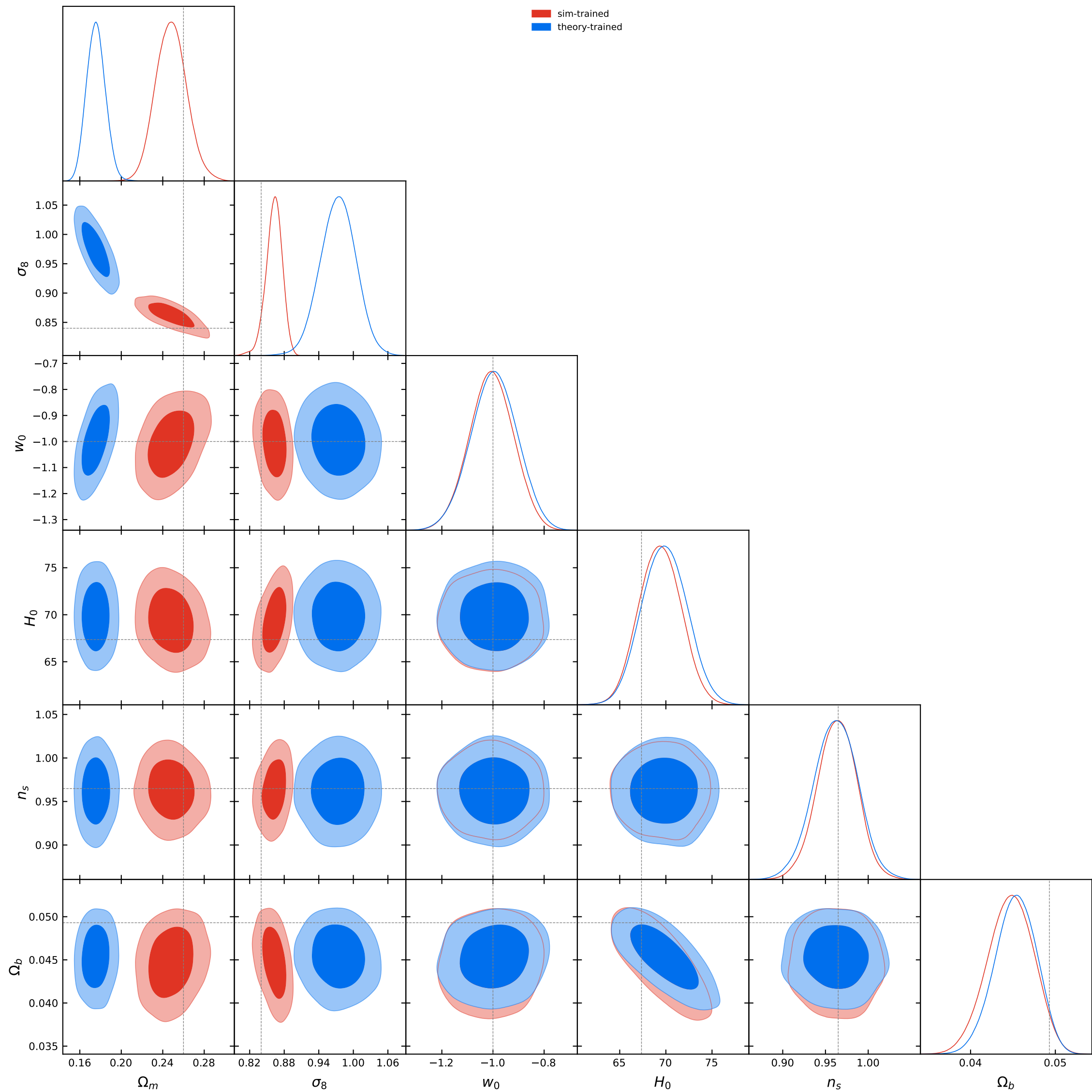
L1 NPE contours: sim vs theory, theta30, cut=aminm0p01_amaxp0p01
