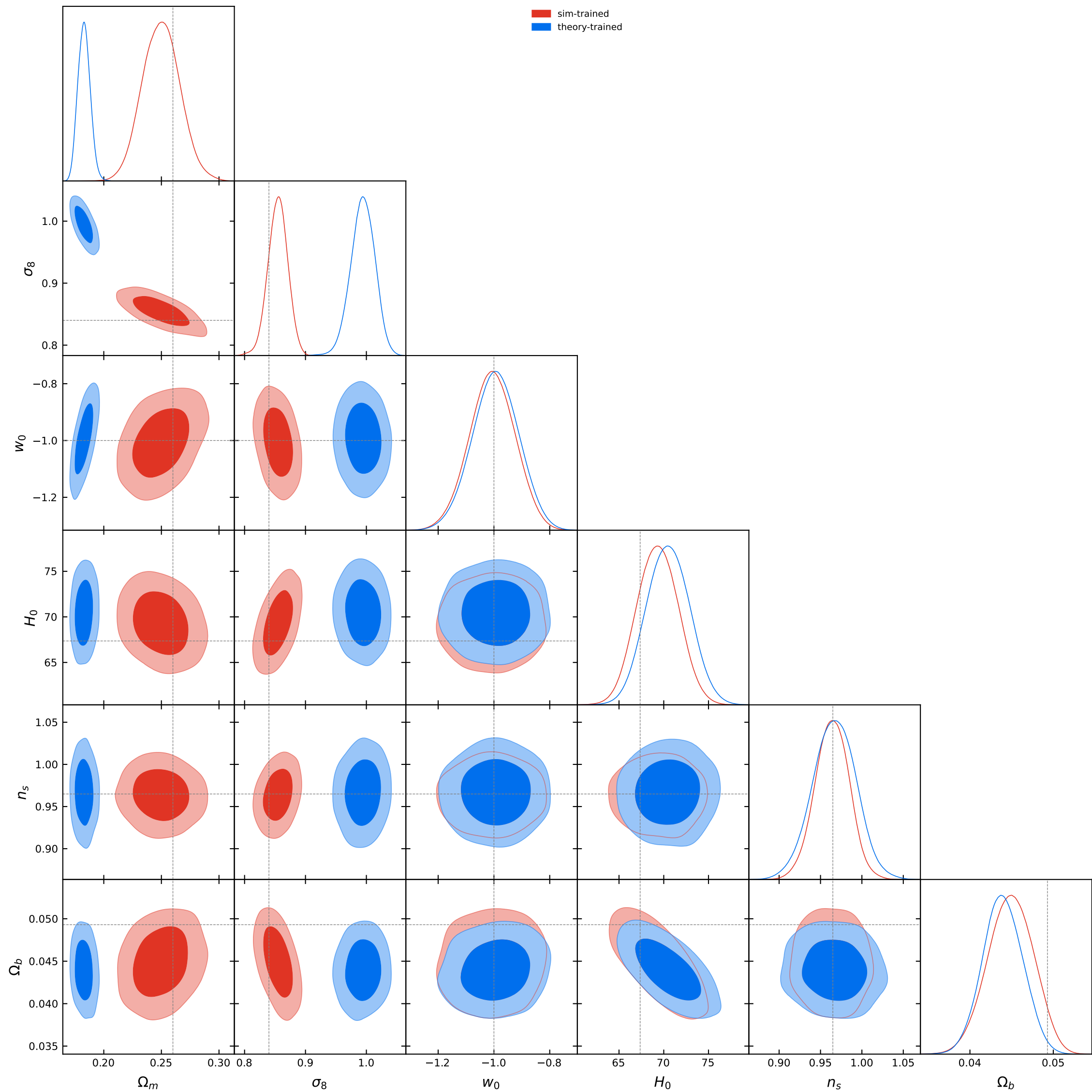
L1 NPE contours: sim vs theory, theta30, cut=aminm0p01_amaxp0p01_dcrm
