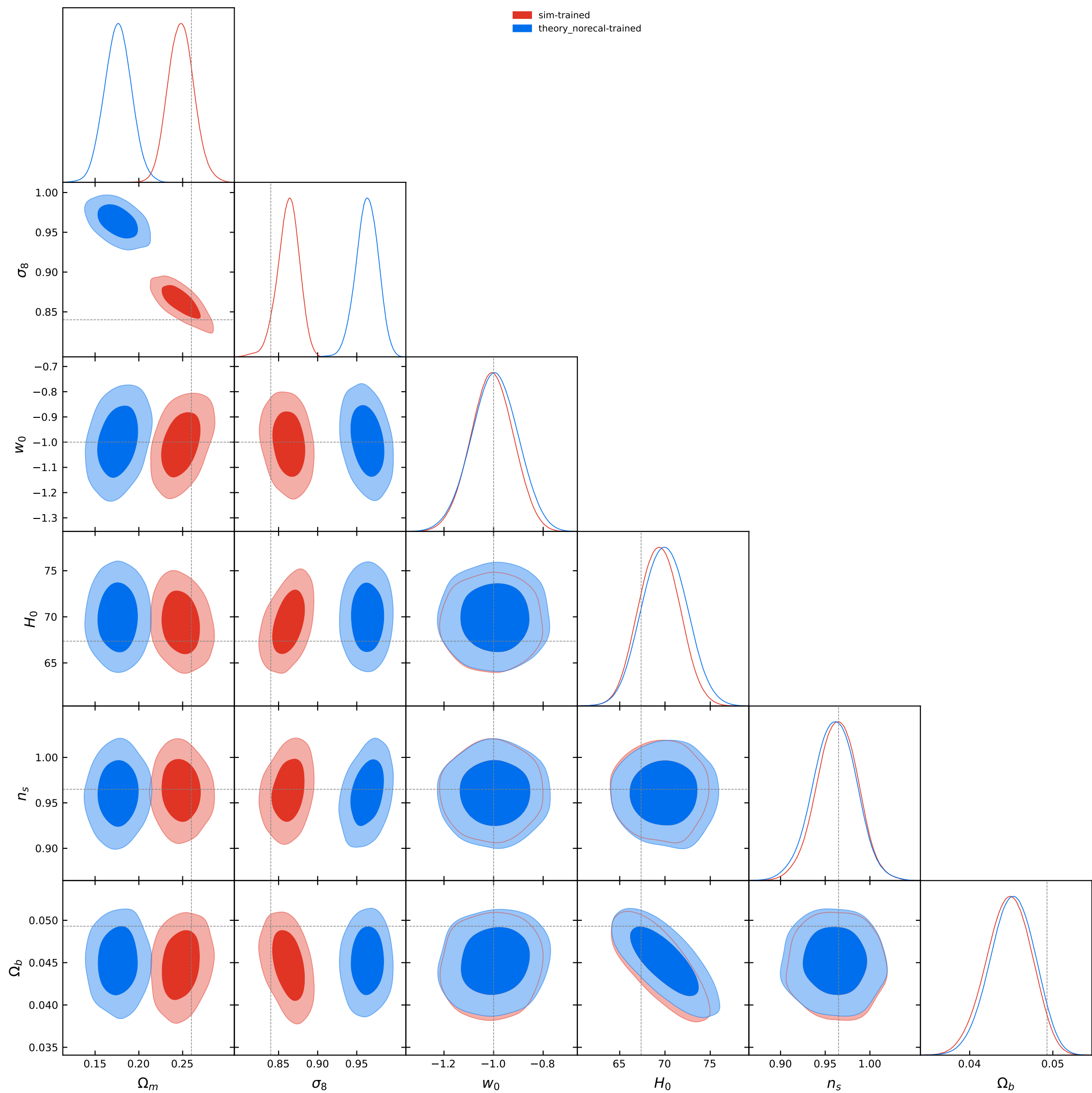
L1 NPE contours: sim vs theory_norecal, theta30, cut=aminm0p01_amaxp0p01_norecal
