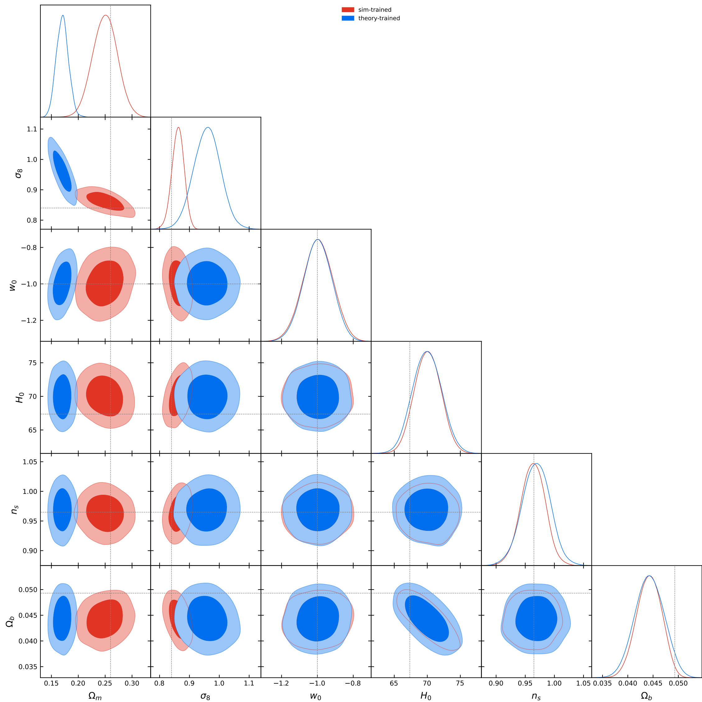
L1 NPE contours: sim vs theory, theta30, cut=dcrm
