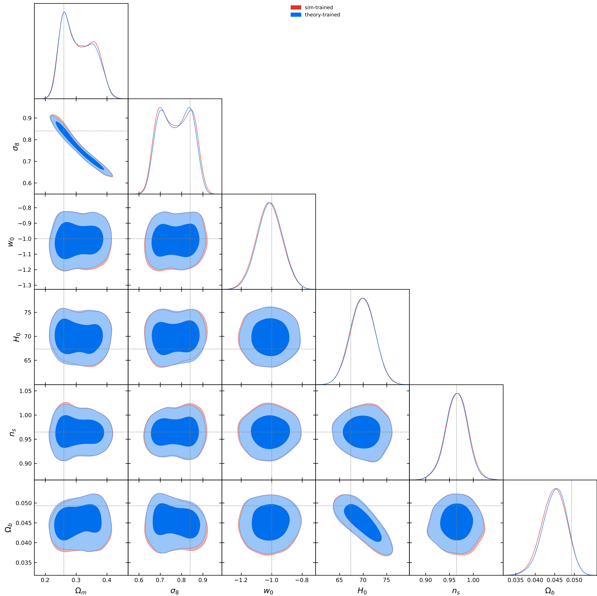
L1 NPE contours: sim vs theory, theta40, cut=aminm0p0006_amaxp0p0006
