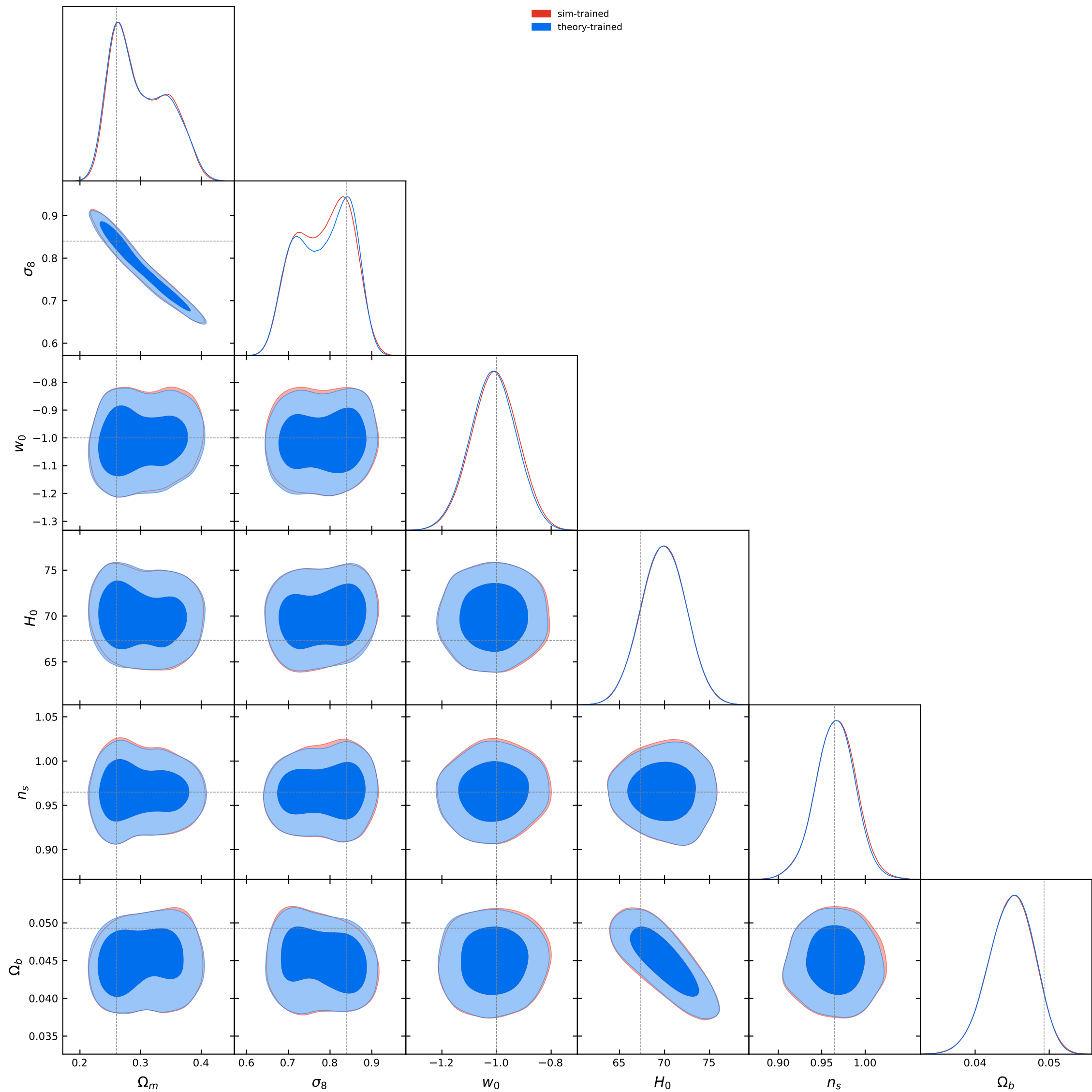
L1 NPE contours: sim vs theory, theta40, cut=aminm0p0013_amaxp0p0006
