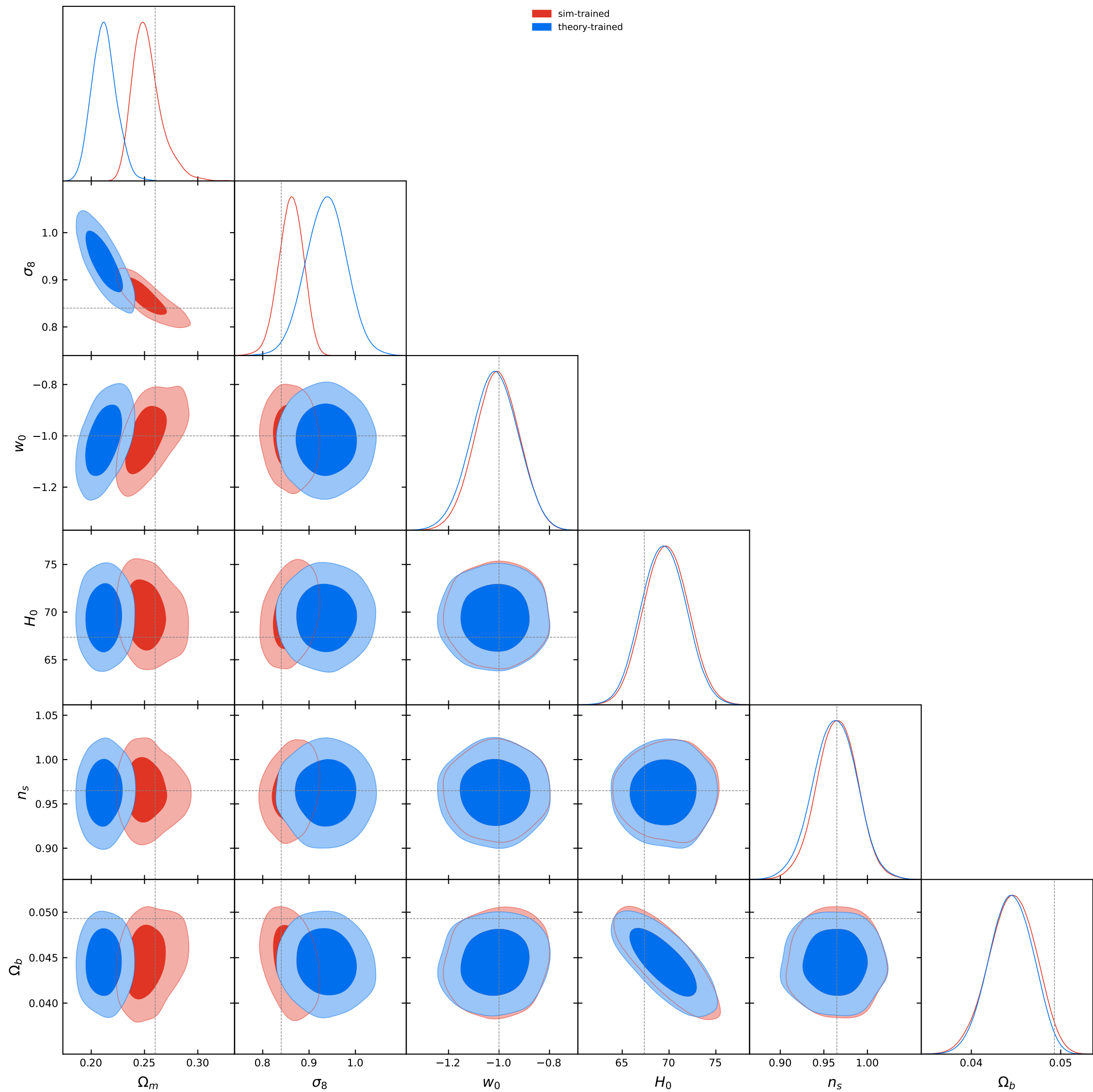
L1 NPE contours: sim vs theory, theta40, cut=aminm0p0113_amaxp0p0113
