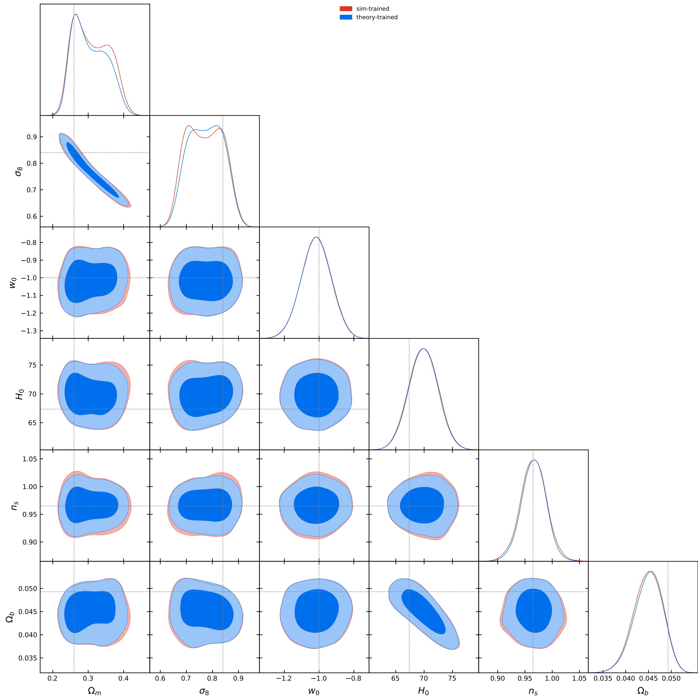
L1 NPE contours: sim vs theory, theta50, cut=aminm0p0005_amaxp0p0005
