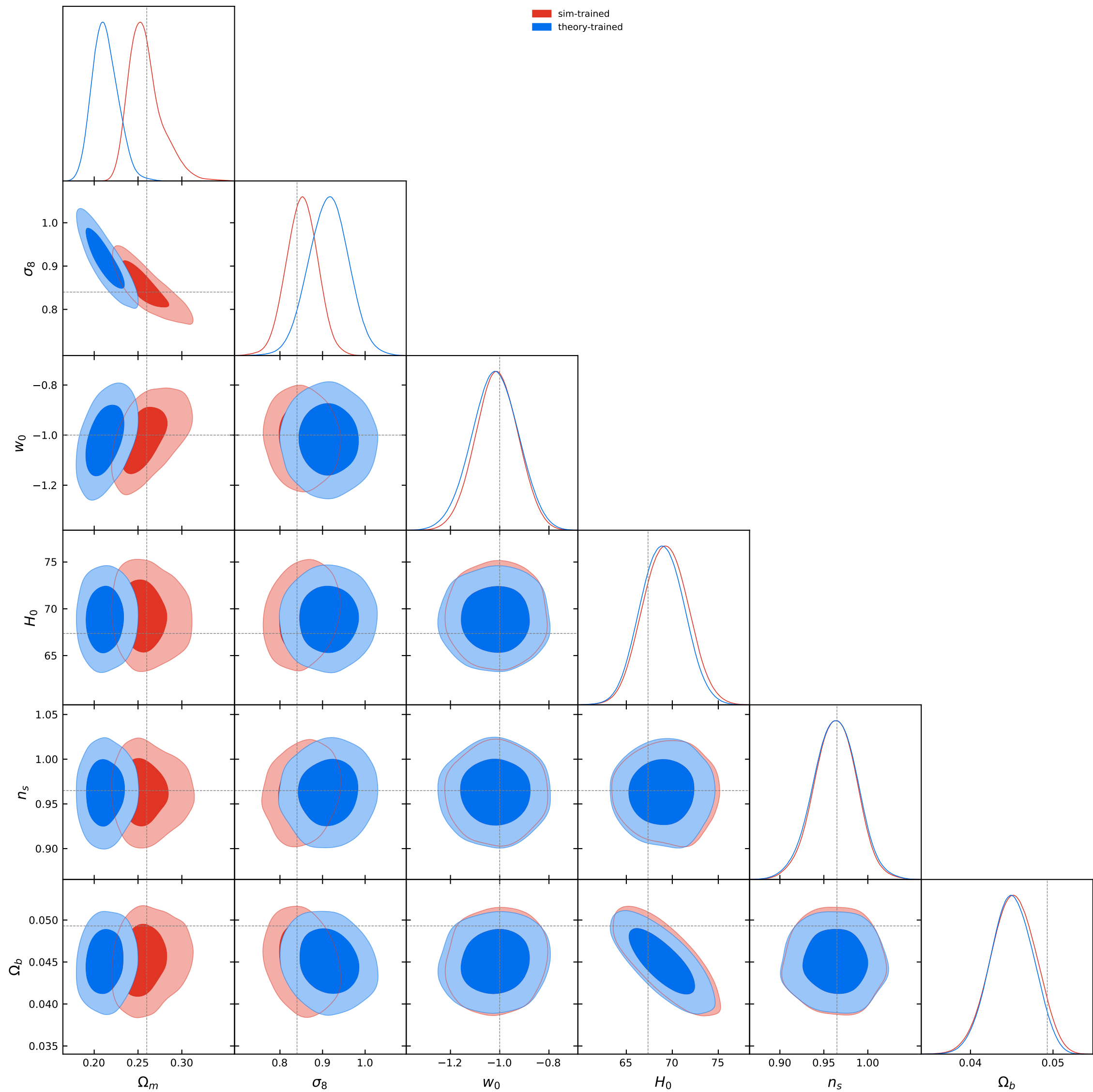
L1 NPE contours: sim vs theory, theta50, cut=aminm0p0103_amaxp0p0103
