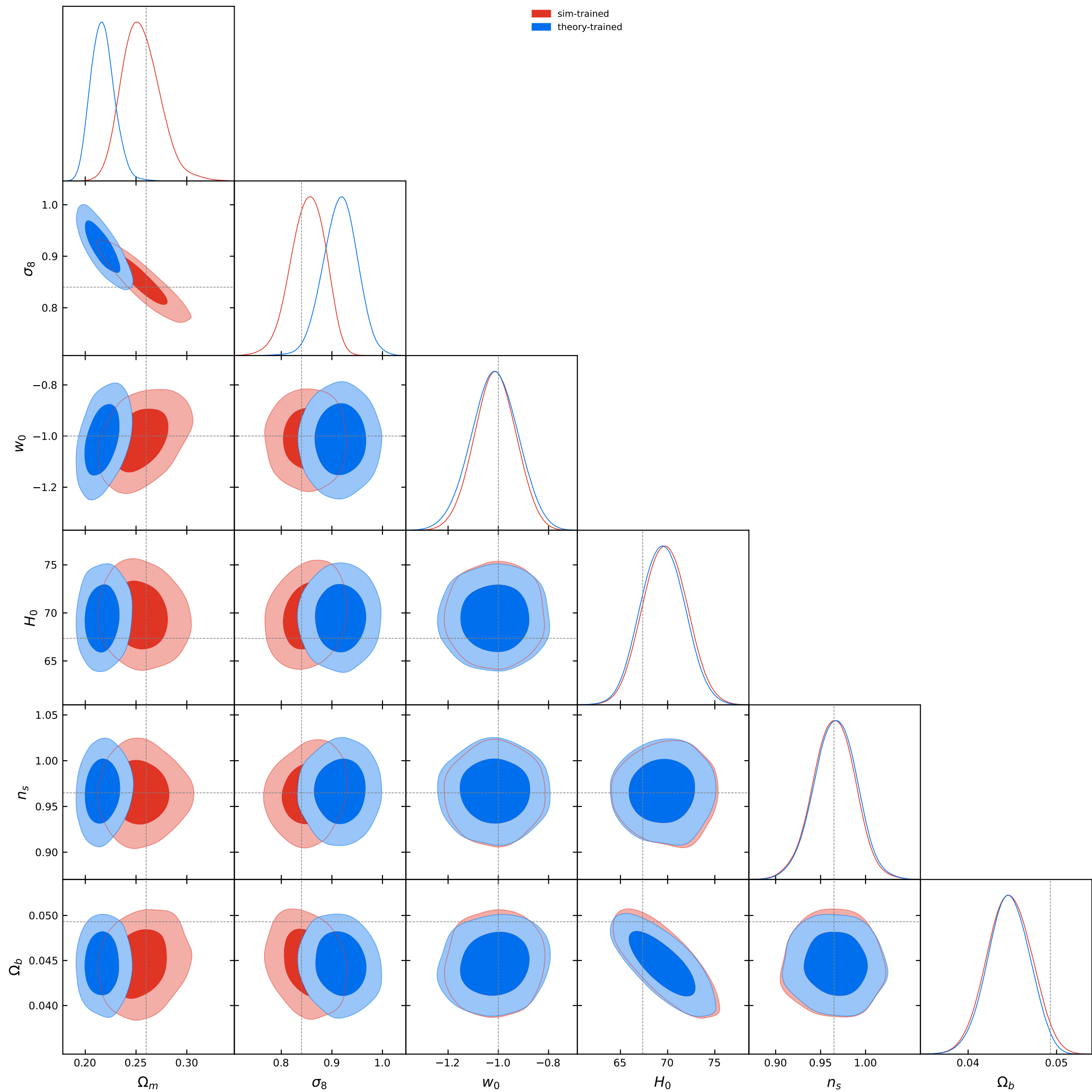
L1 NPE contours: sim vs theory, theta50, cut=full
