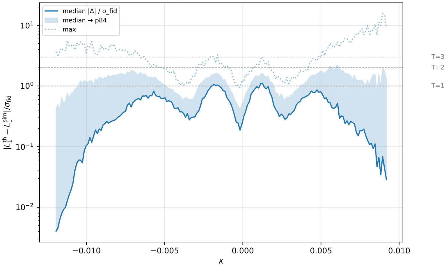
L1 residual per-cosmo distribution, \theta=60'
