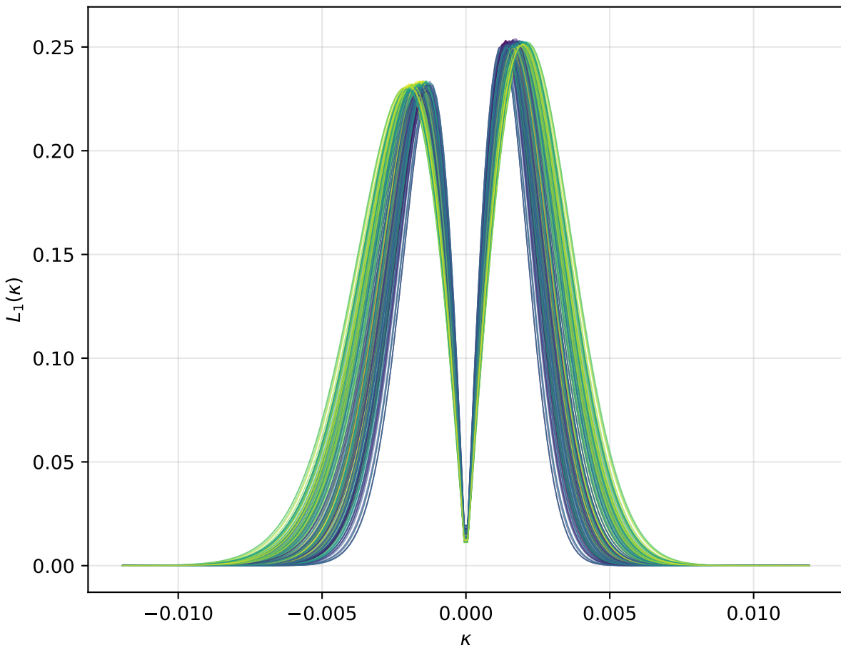
Theory L_1 (per cosmology), \theta=60.0'
