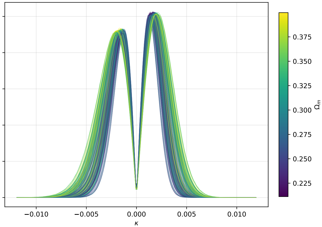
Sim L_1 mean (per cosmology, over 7 perms), \theta=60.0'
