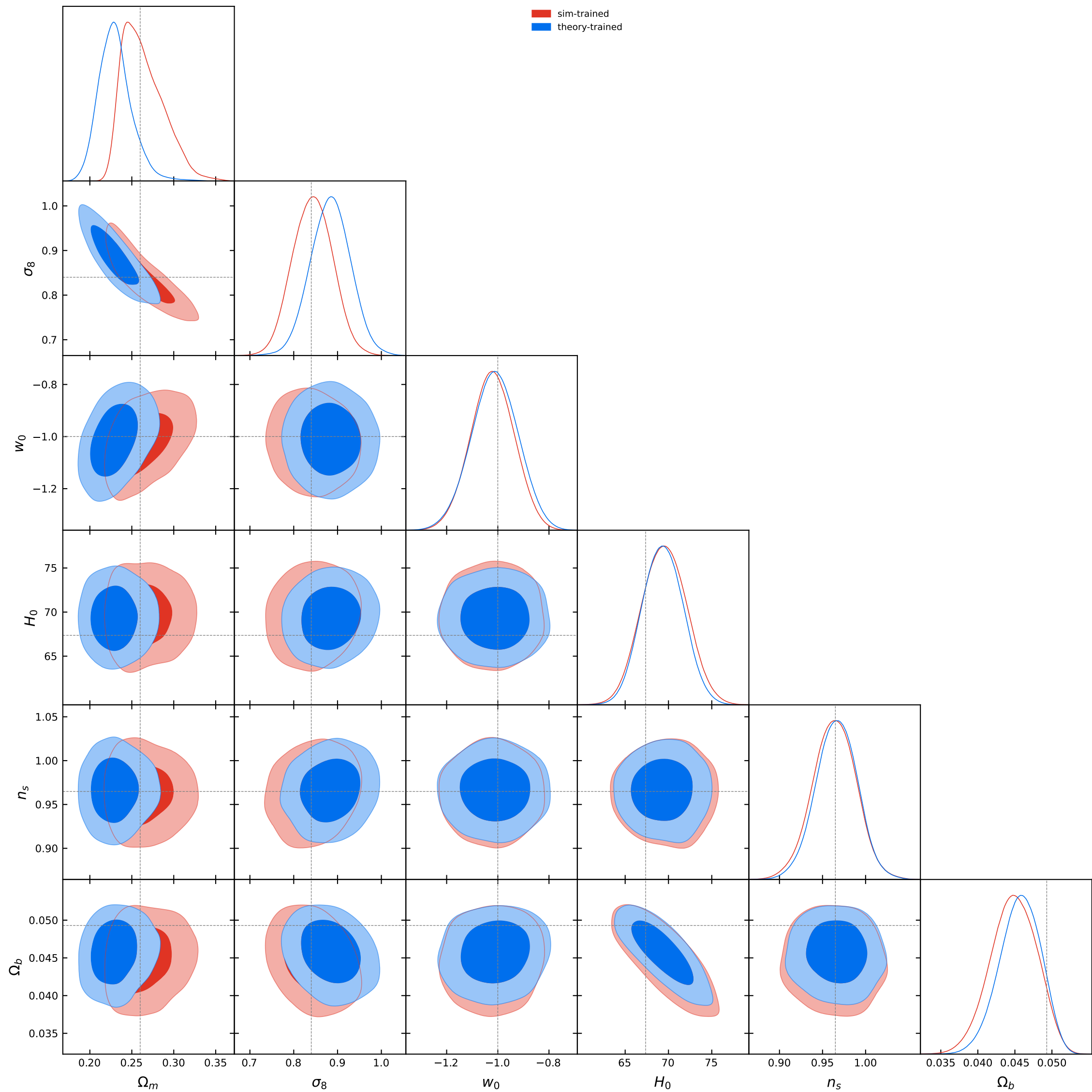
L1 NPE contours: sim vs theory, theta60, cut=aminm0p0092_amaxp0p0092
