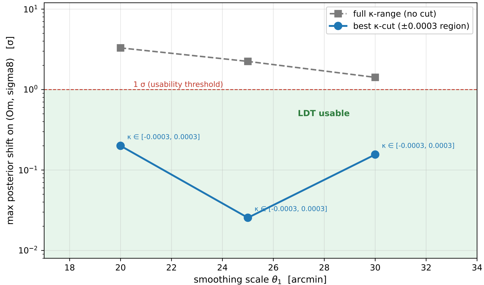
LDT \ell_1 -norm posterior bias vs \theta — BNT bin 4 (bnt4)
