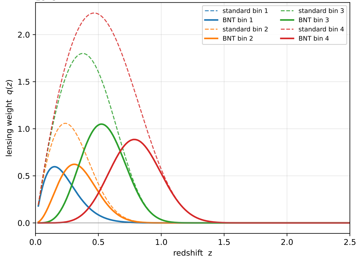
Standard vs BNT lensing kernels (cosmoGRID, fiducial)
